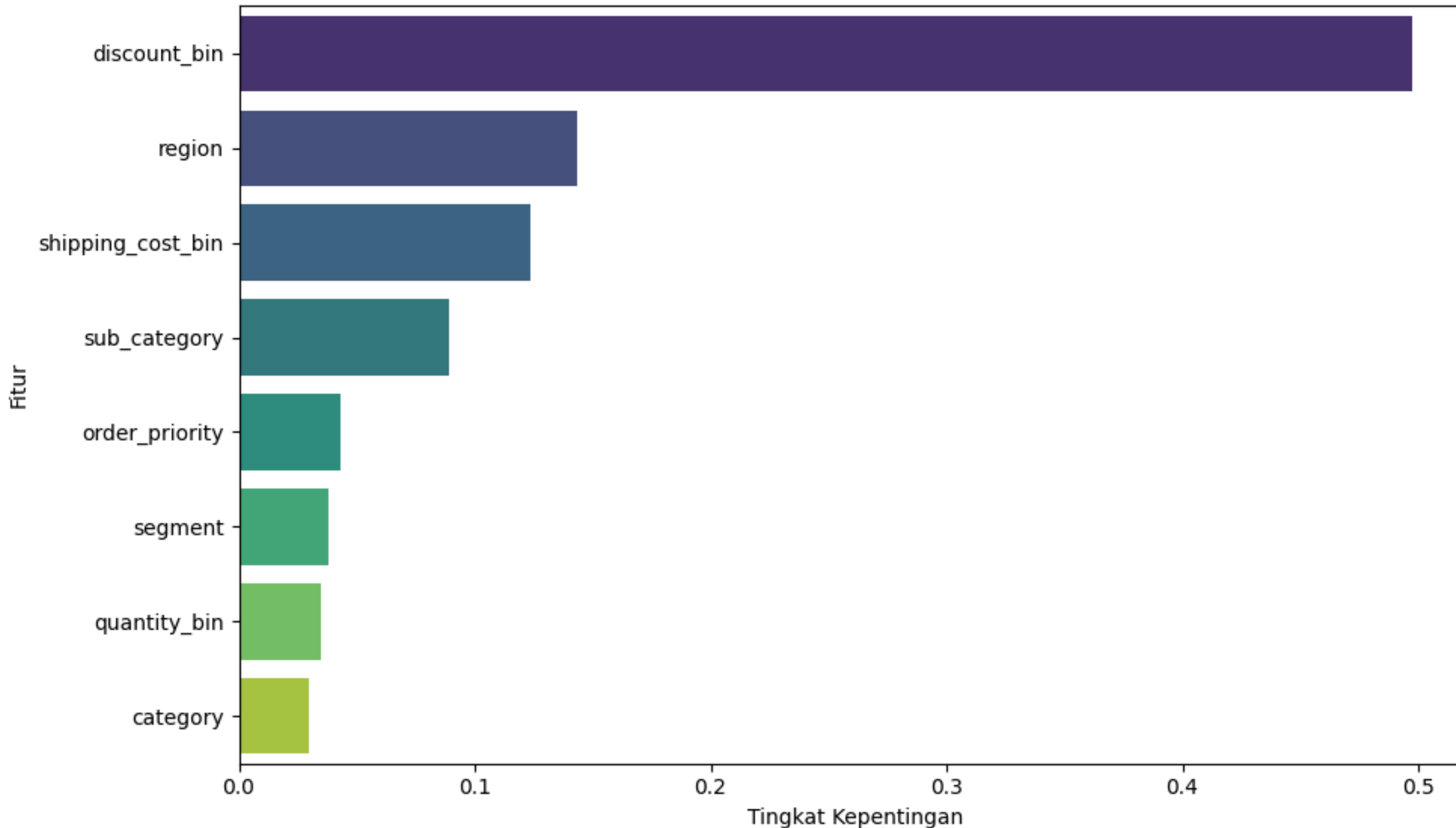
Feature Importance (Random Forest)
