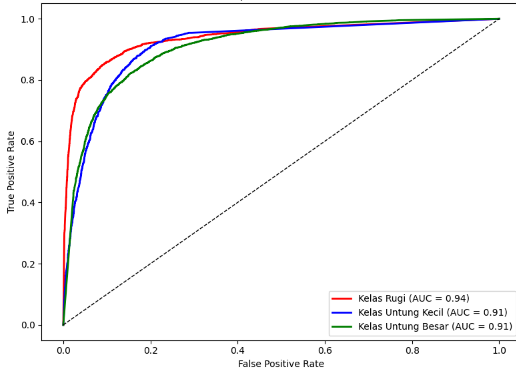
ROC Curve per Kelas (Random Forest)
