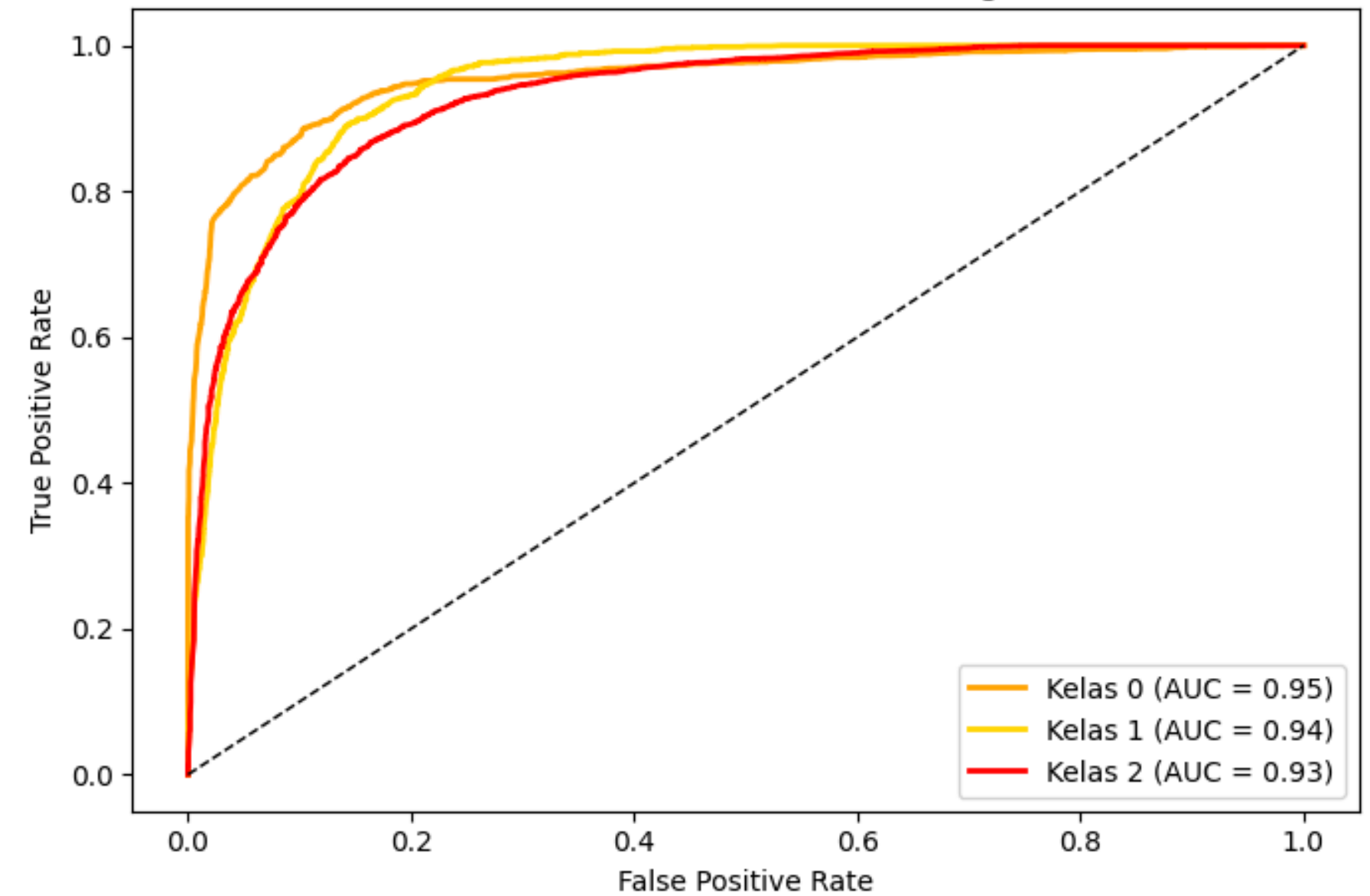
ROC Curve - Gradient Boosting
