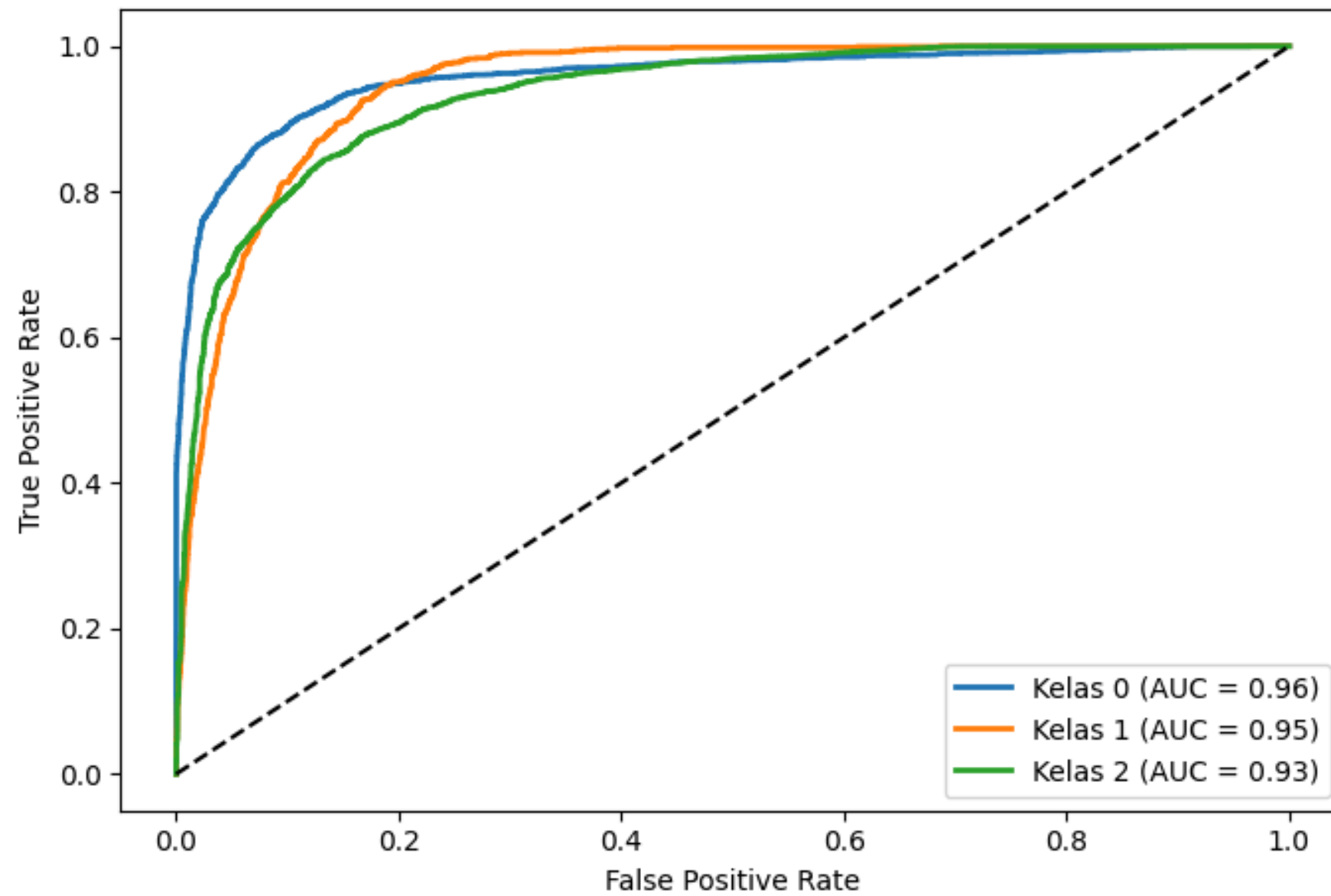
ROC Curve - XGBoost
