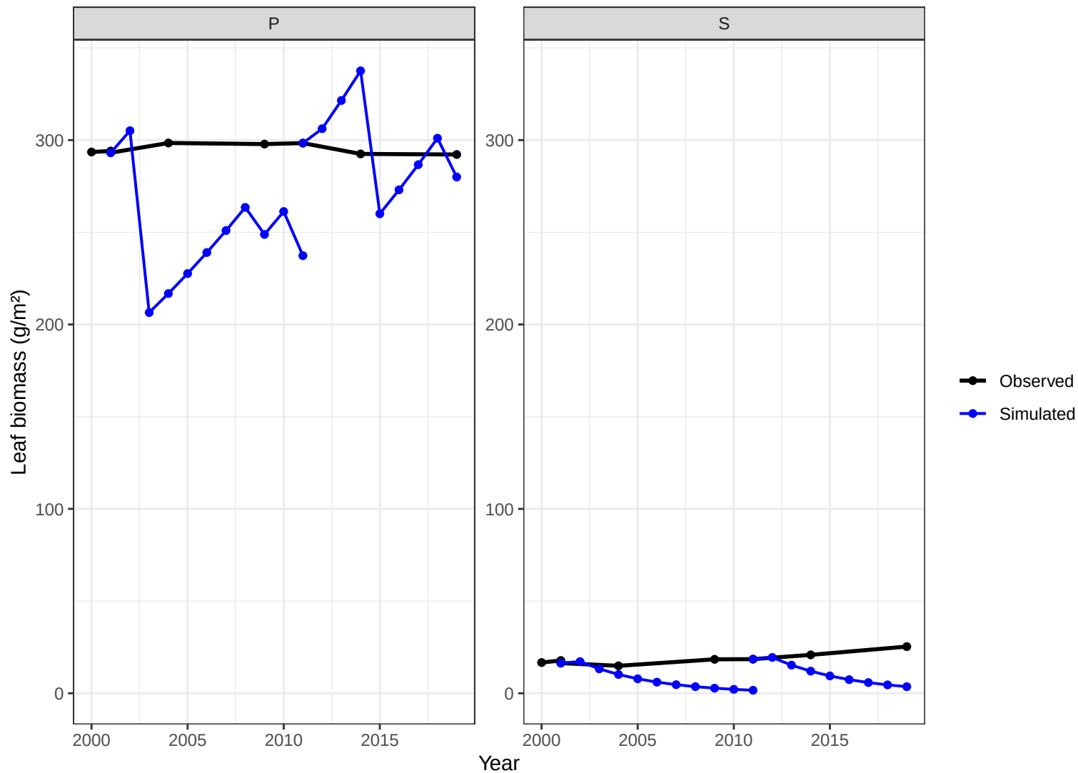
Site CHS01 – leaf biomass obs vs simulated
