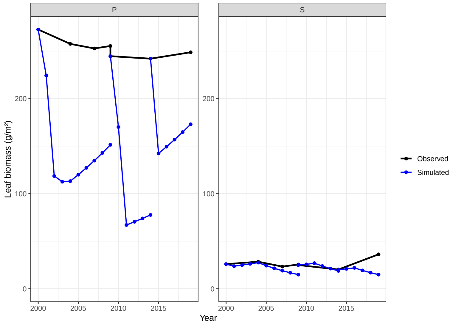
Site CHS58 – leaf biomass obs vs simulated
