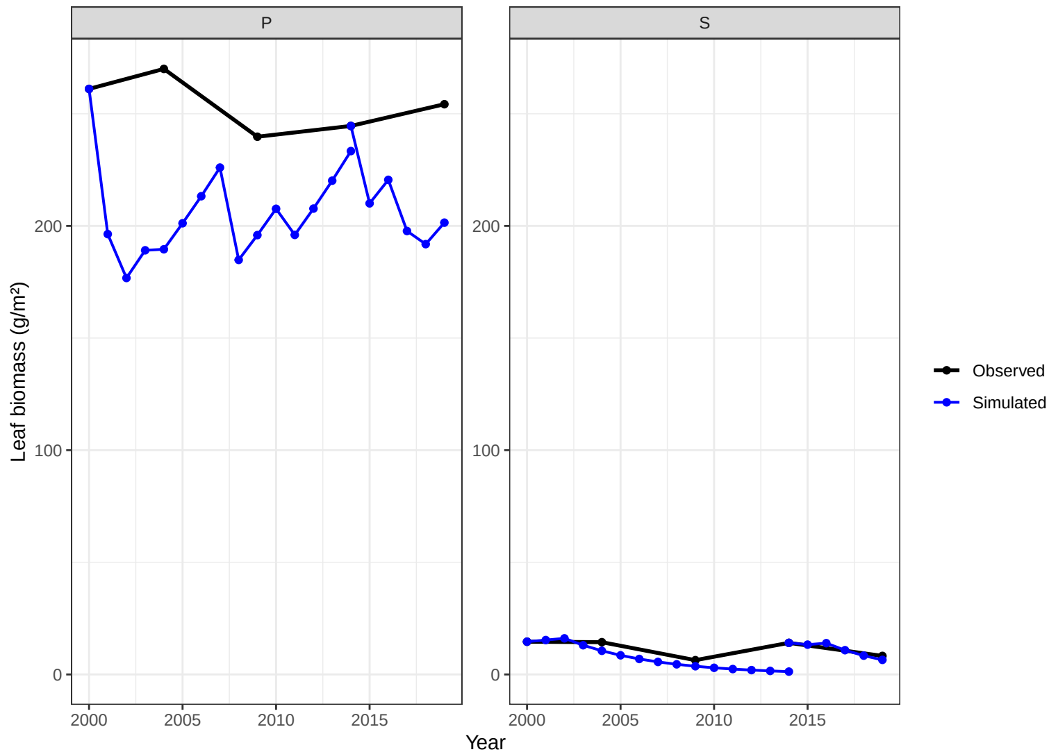
Site CHS57b – leaf biomass obs vs simulated
