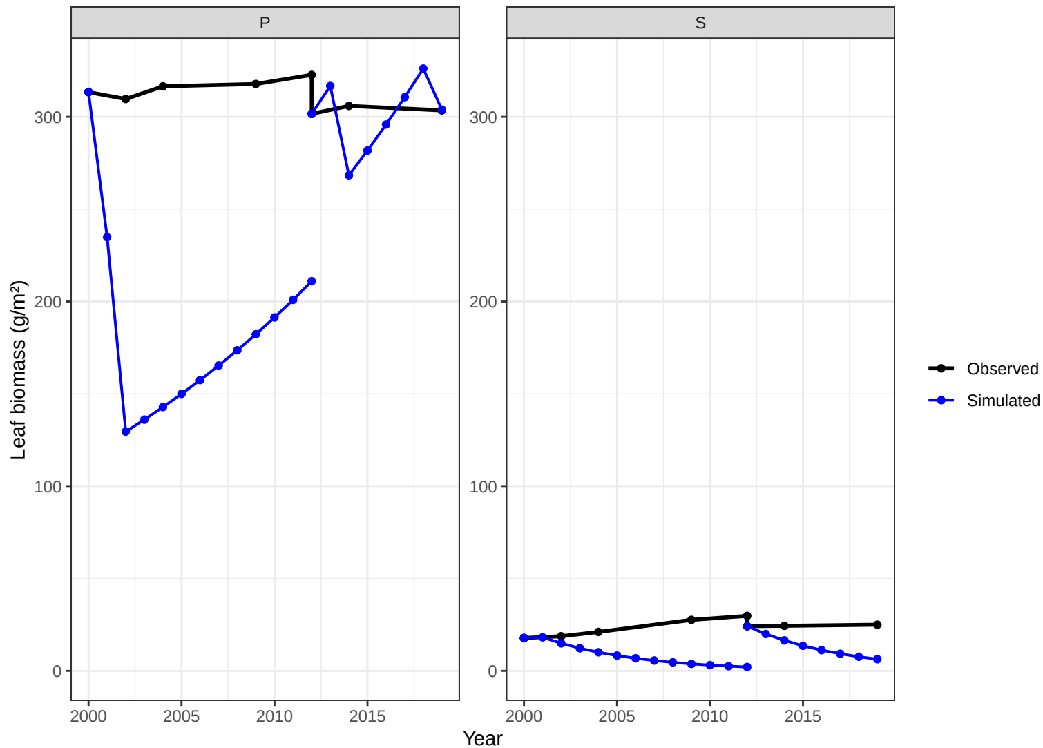
Site CHS21 – leaf biomass obs vs simulated
