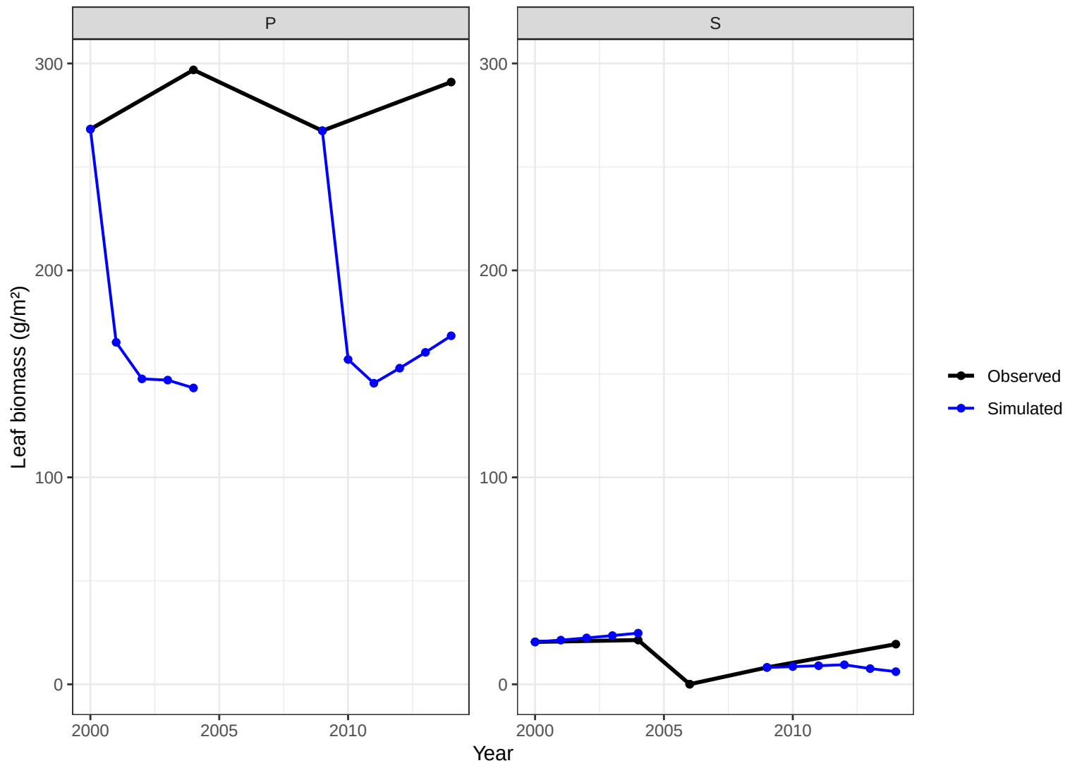
Site CHS27 – leaf biomass obs vs simulated
