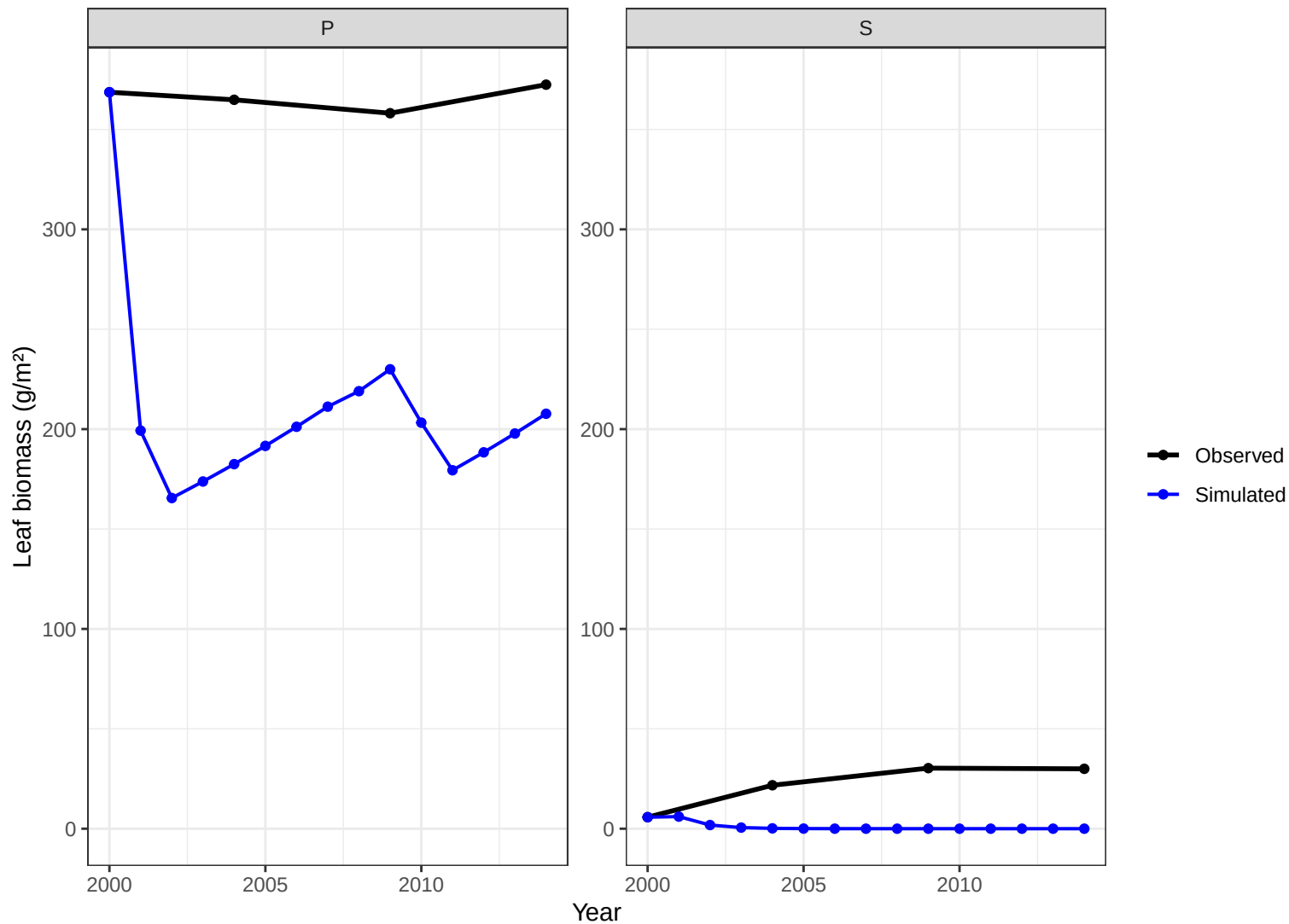
Site CHS60 – leaf biomass obs vs simulated
