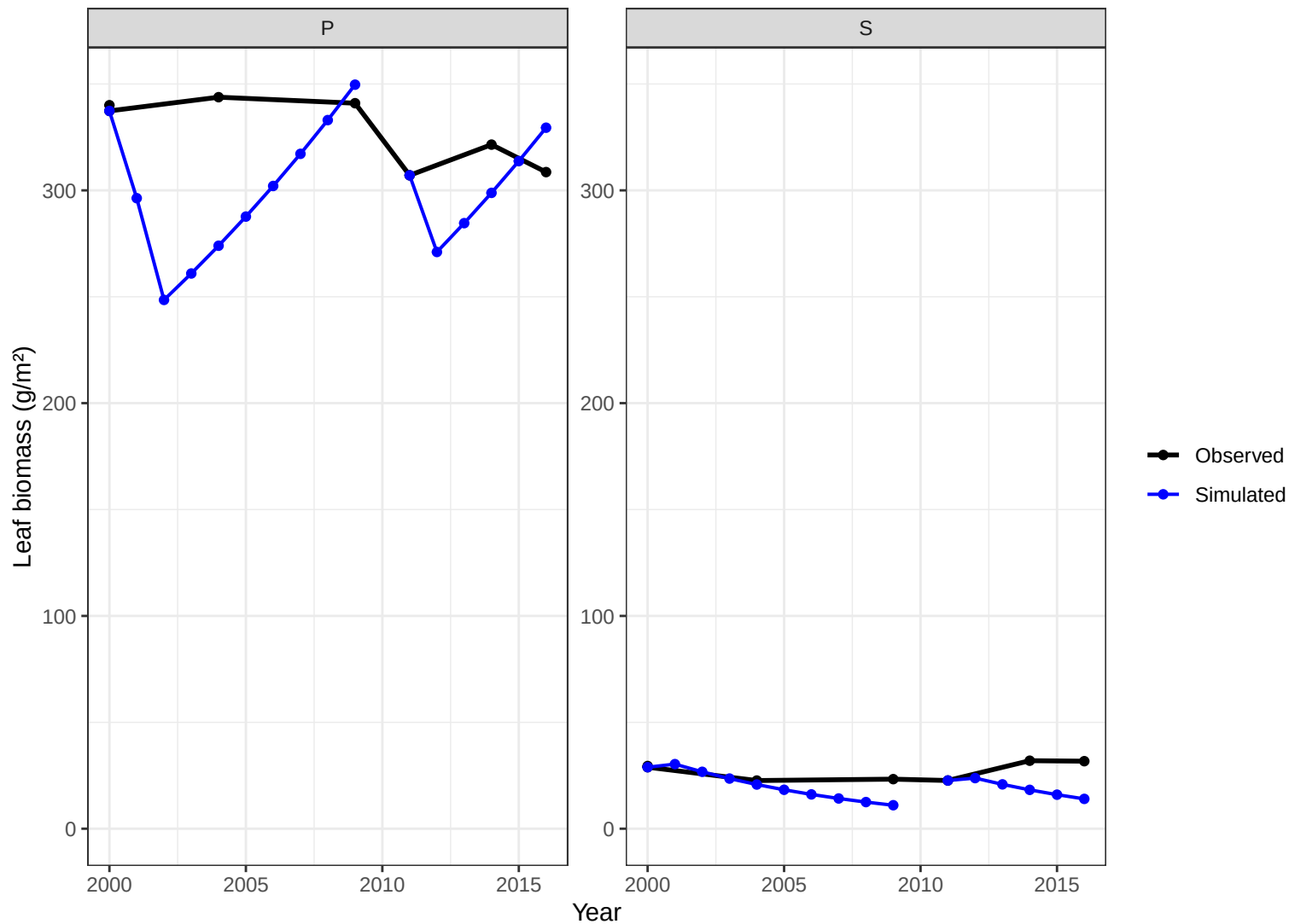
Site CHS35 – leaf biomass obs vs simulated
