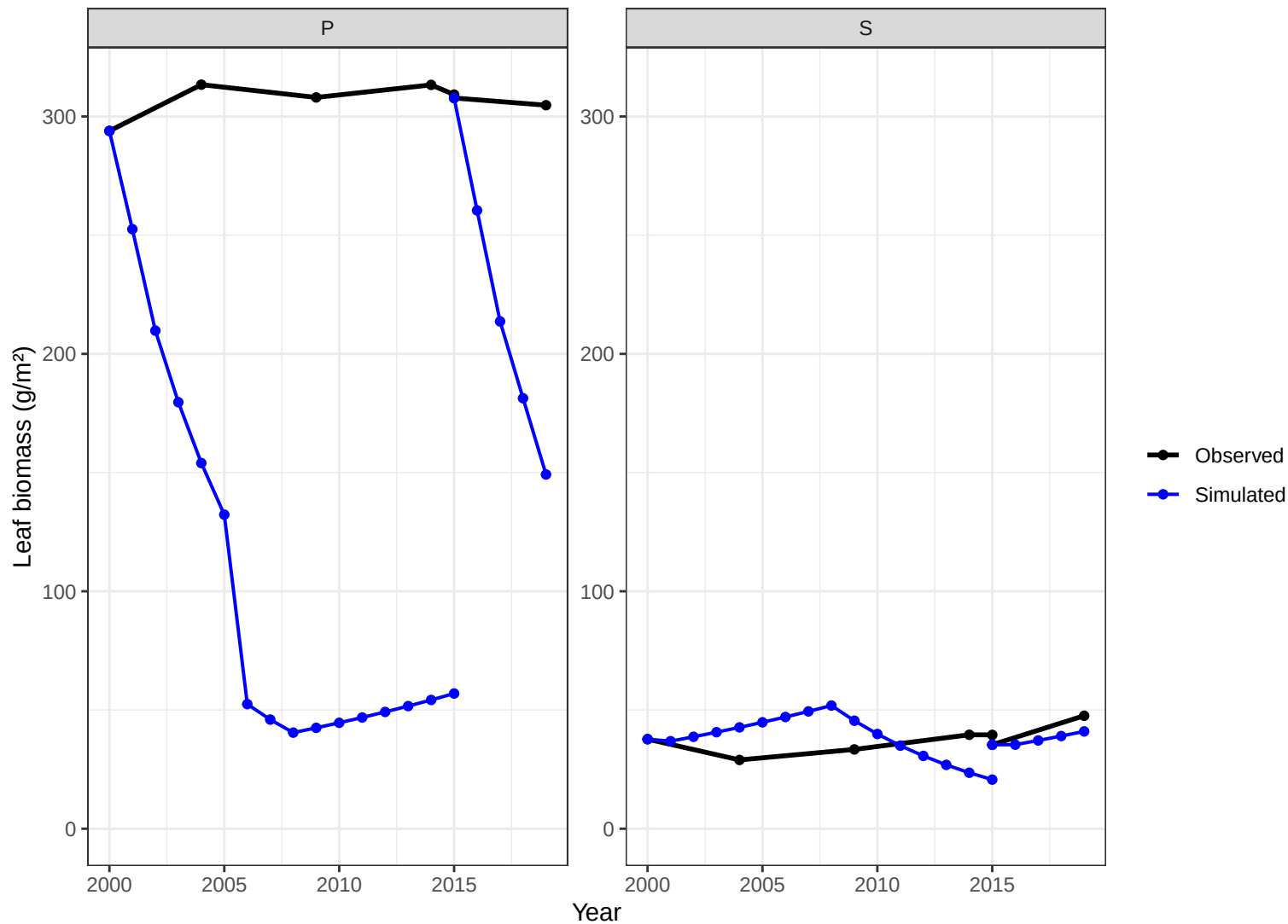
Site CHS86 – leaf biomass obs vs simulated
