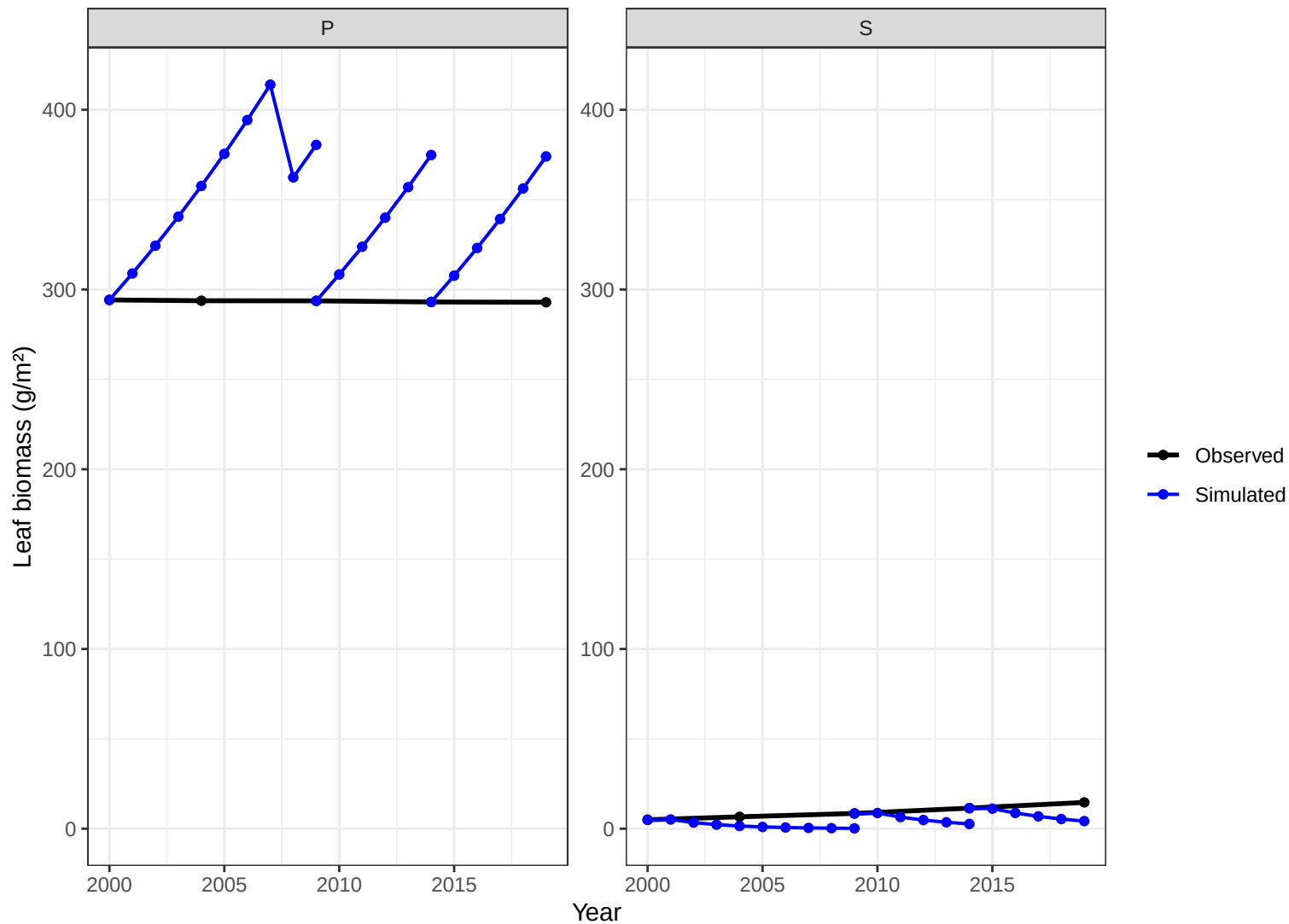
Site CHS81 – leaf biomass obs vs simulated
