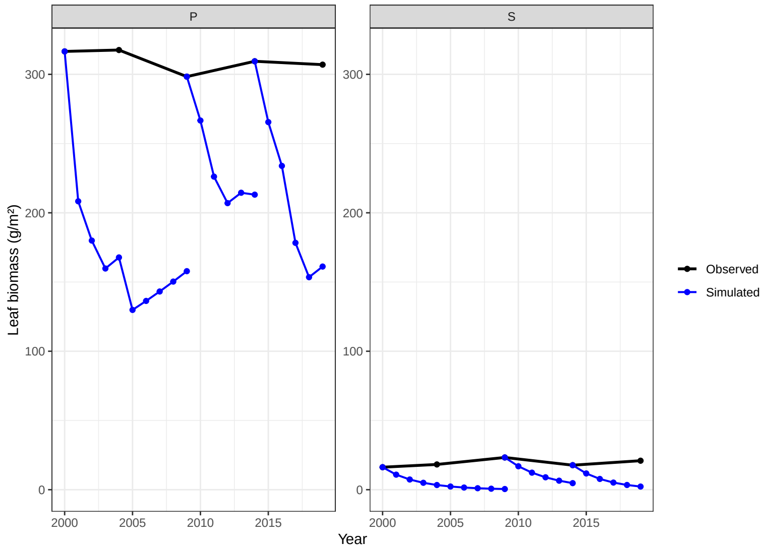
Site CHS03 – leaf biomass obs vs simulated
