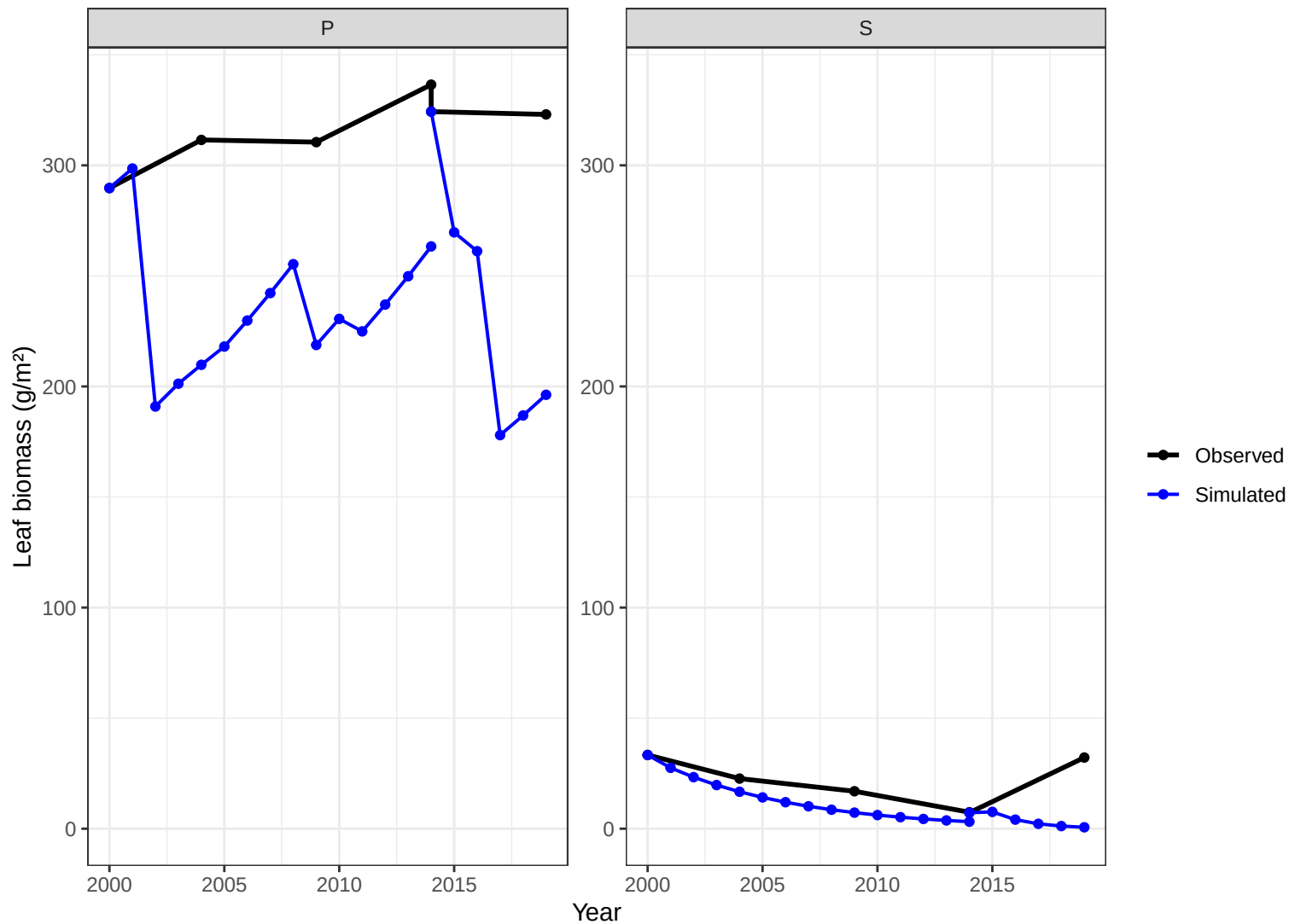
Site CHS57a – leaf biomass obs vs simulated
