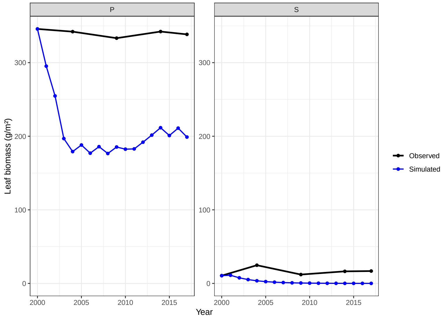
Site CHS61 – leaf biomass obs vs simulated
