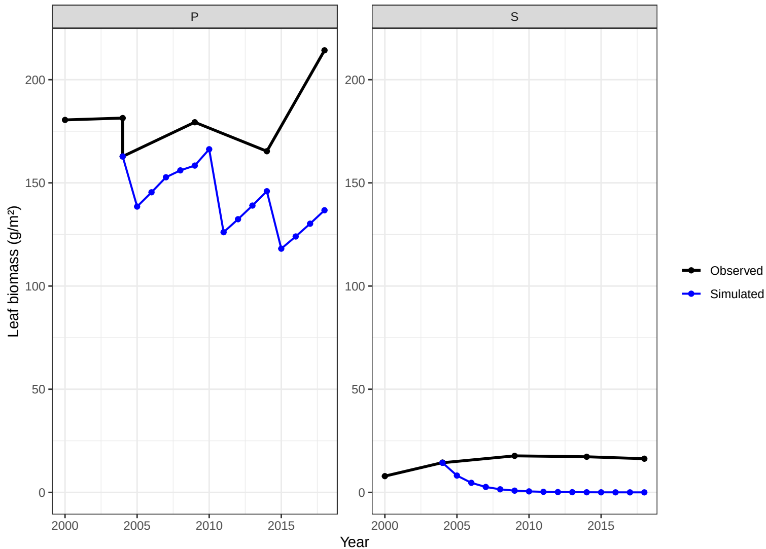
Site CHS68 – leaf biomass obs vs simulated
