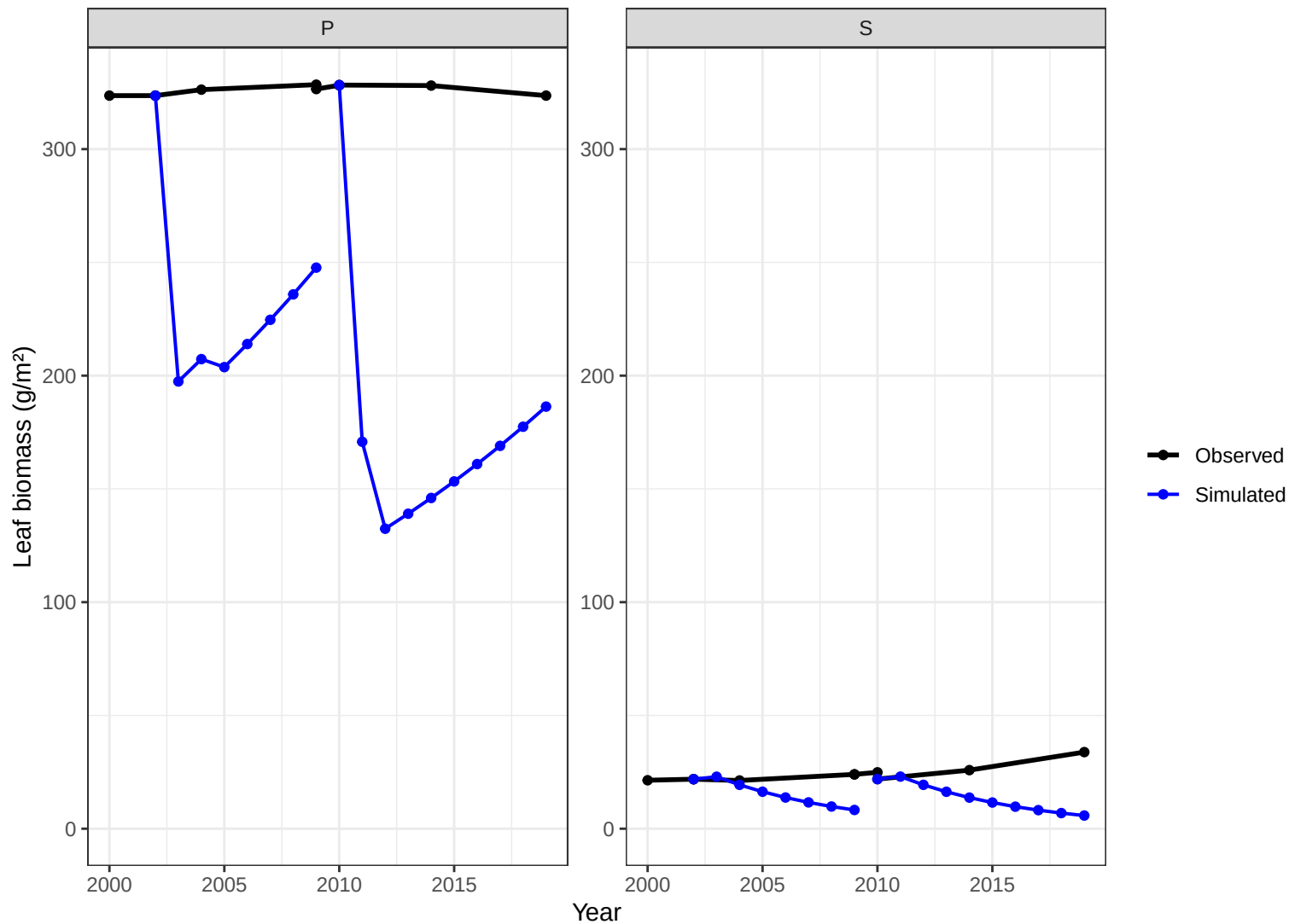
Site CHS41 – leaf biomass obs vs simulated
