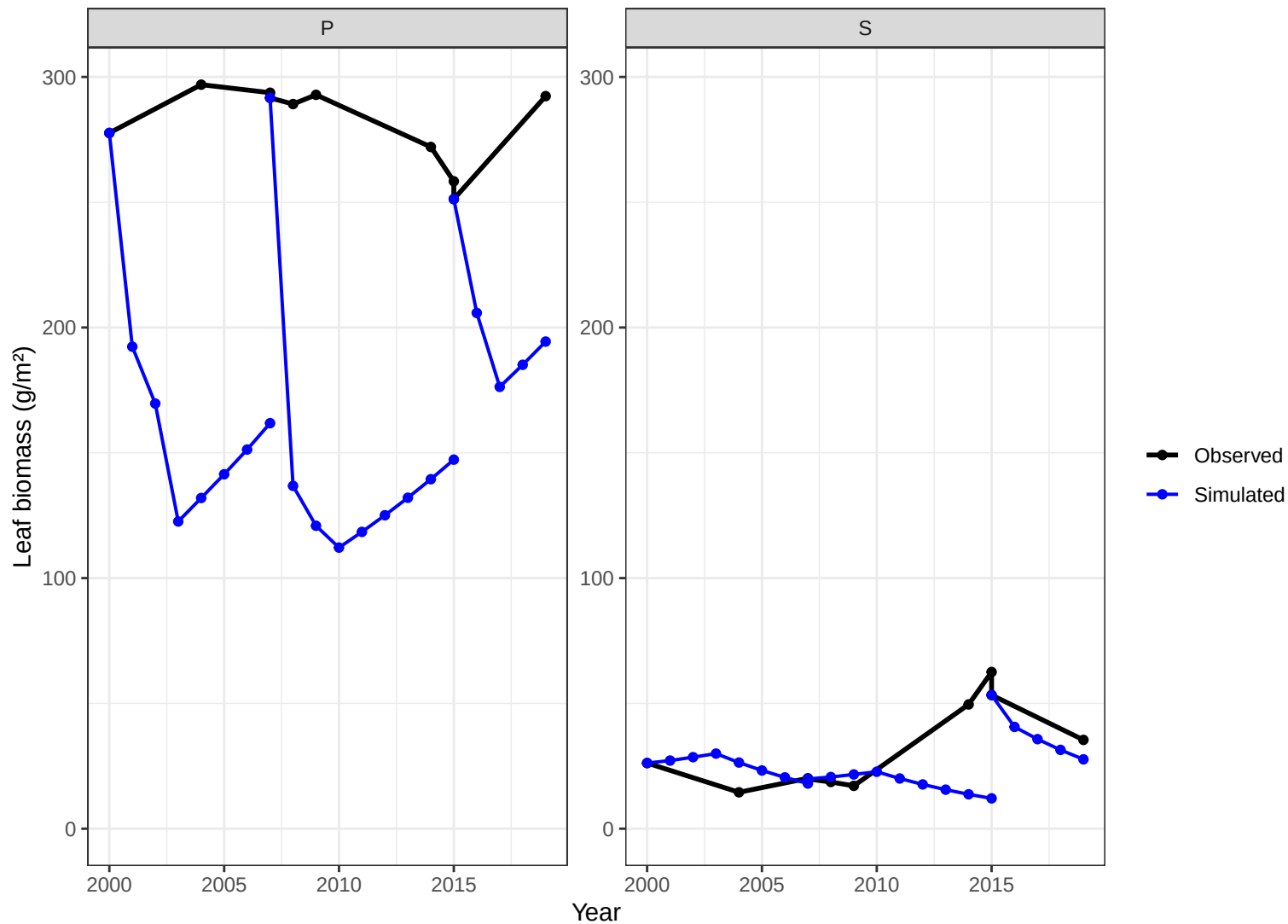
Site CHS72 – leaf biomass obs vs simulated
