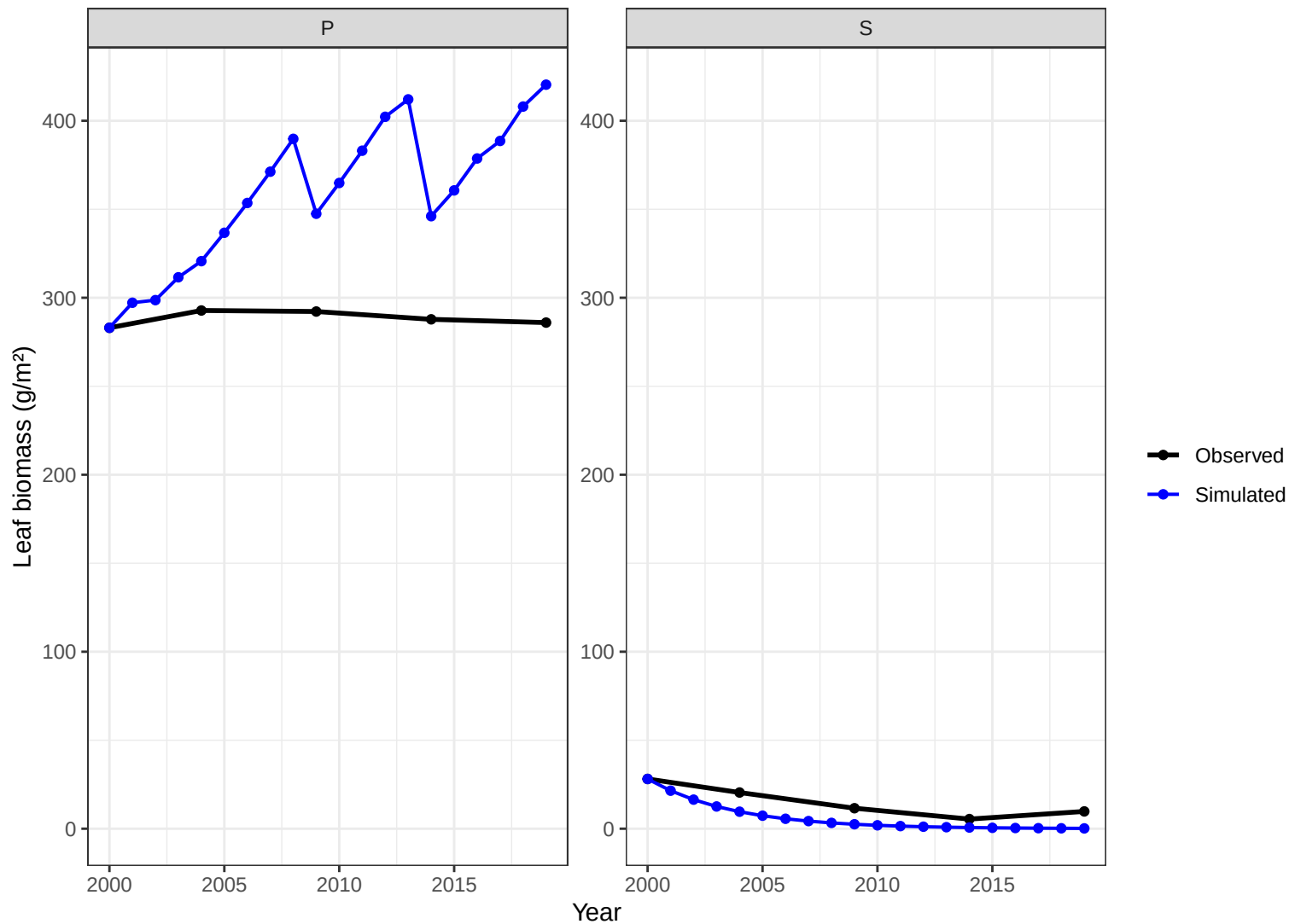
Site CHS88 – leaf biomass obs vs simulated
