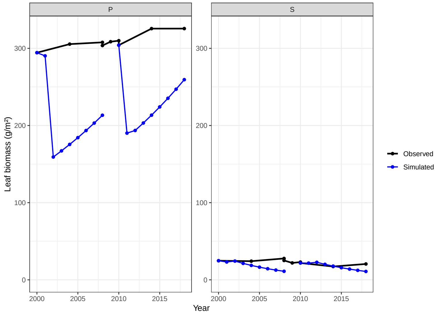
Site CHS10 – leaf biomass obs vs simulated
