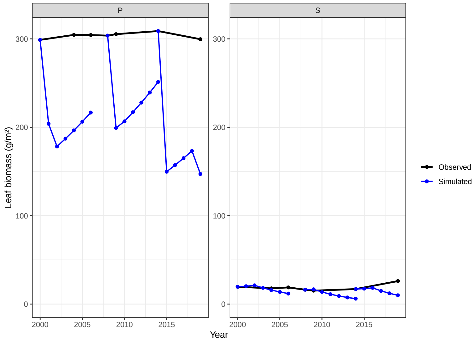
Site CHS18 – leaf biomass obs vs simulated
