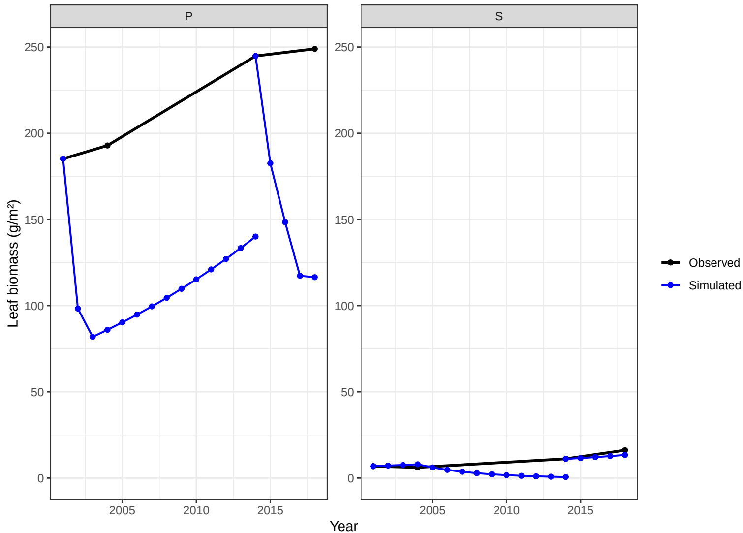
Site CHS51 – leaf biomass obs vs simulated
