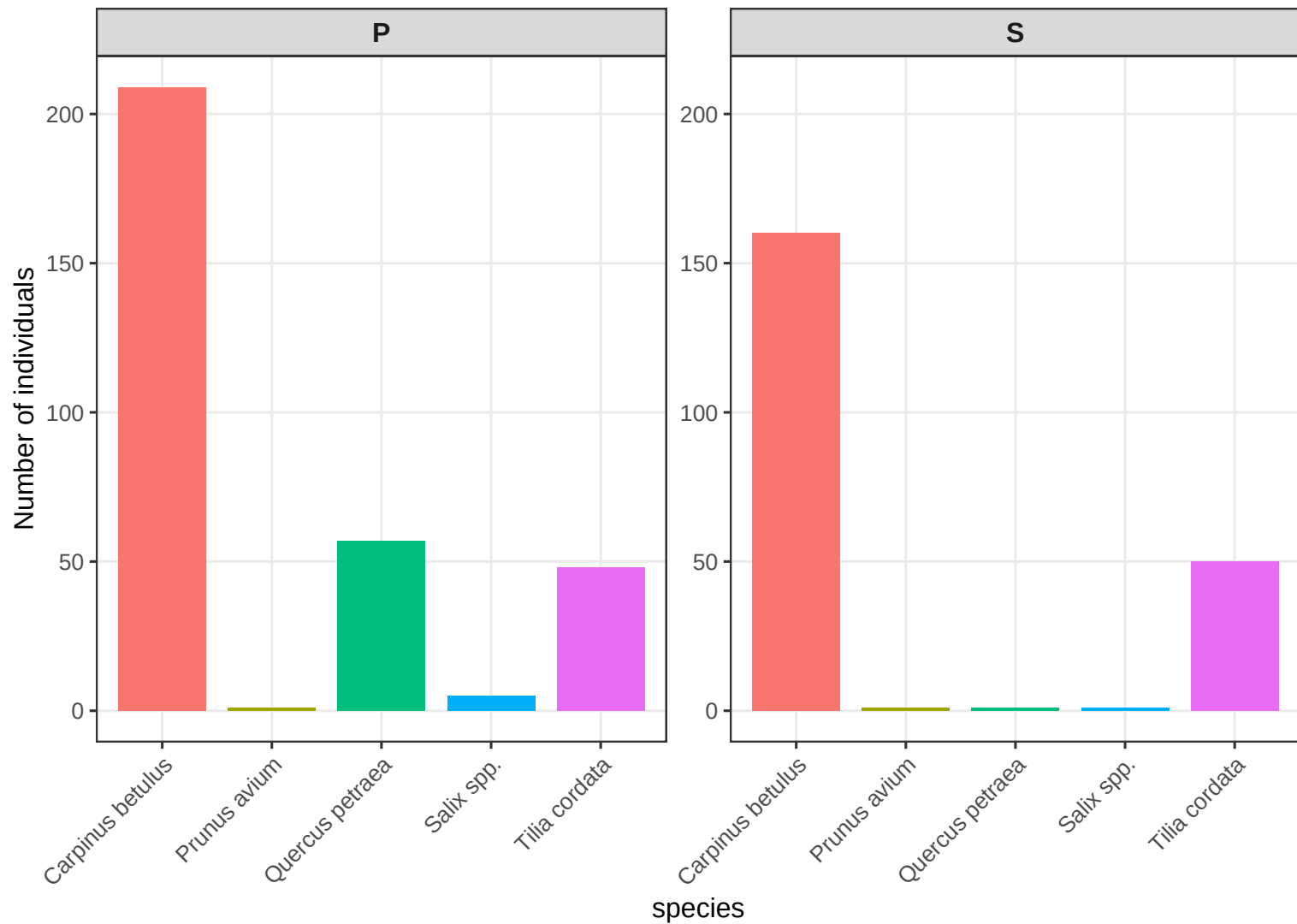
Number of individuals per sp and canopy layer on CHS 68
