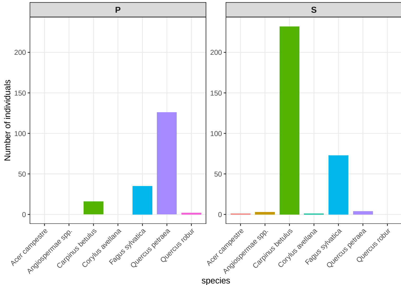
Number of individuals per sp and canopy layer on CHS 21
