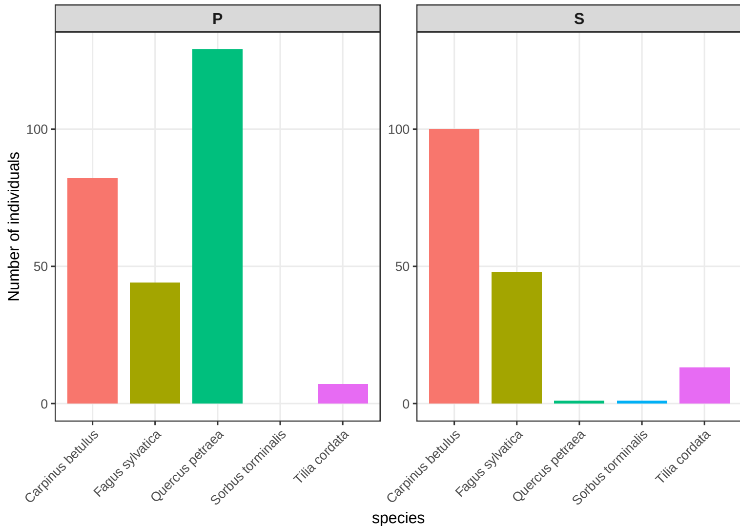
Number of individuals per sp and canopy layer on CHS 57a
