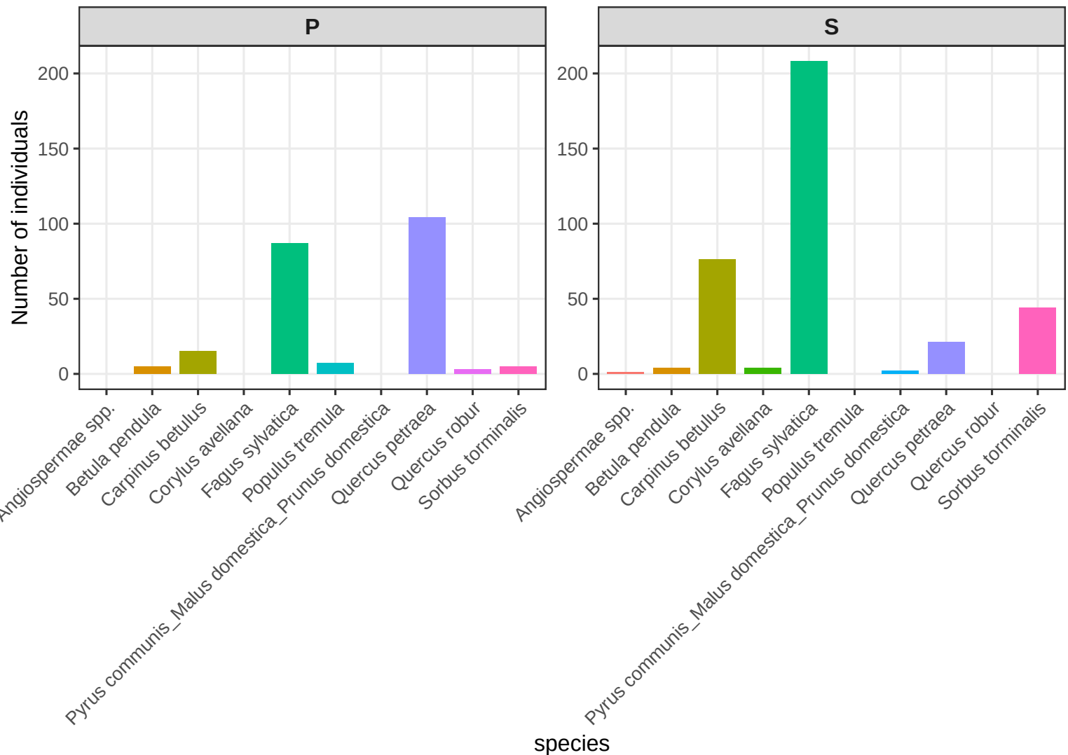
Number of individuals per sp and canopy layer on CHS 10
