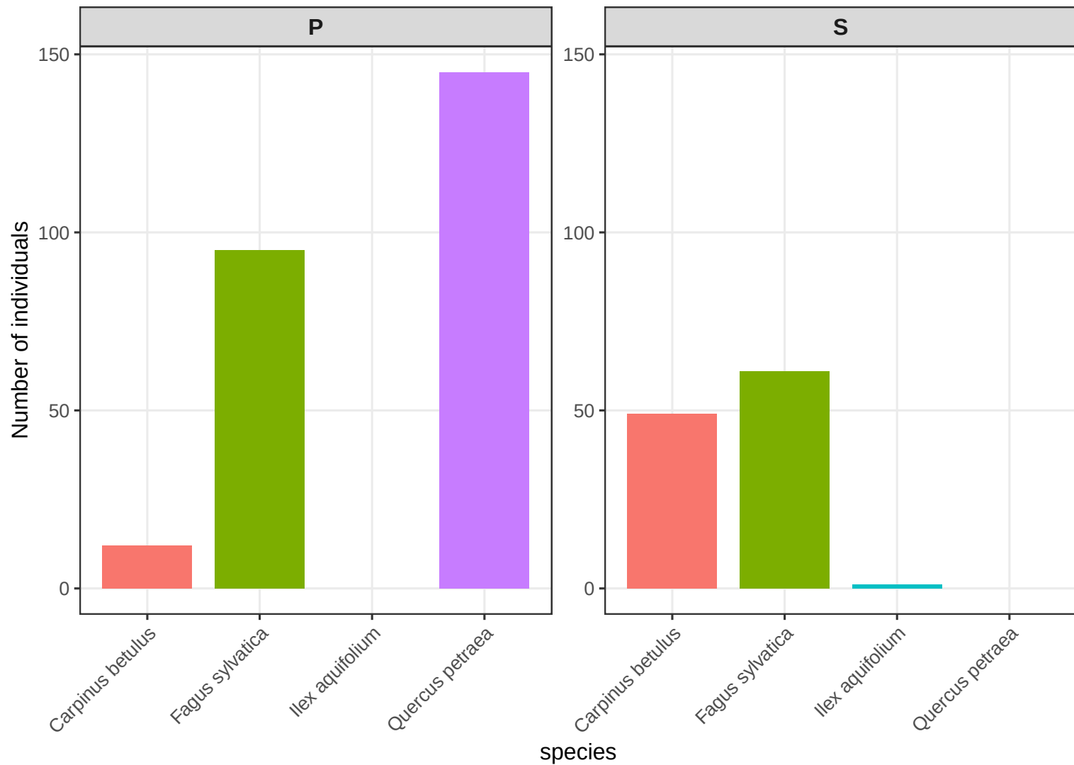
Number of individuals per sp and canopy layer on CHS 61
