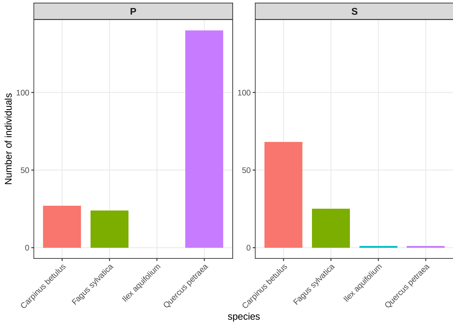
Number of individuals per sp and canopy layer on CHS 03
