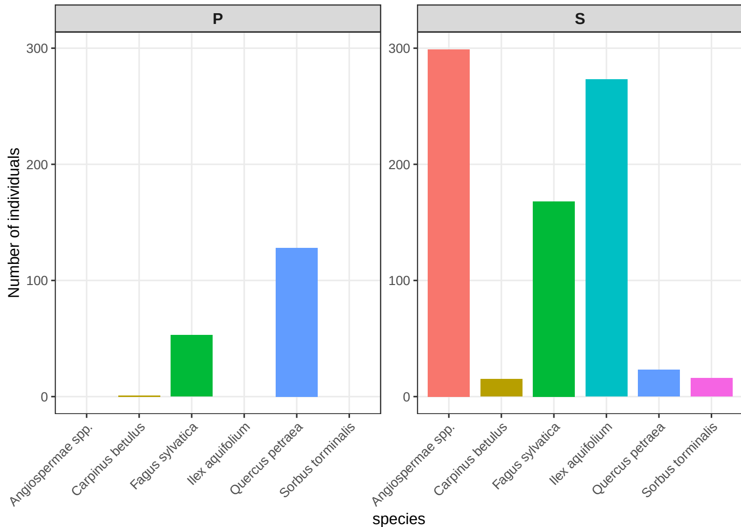
Number of individuals per sp and canopy layer on CHS 86
