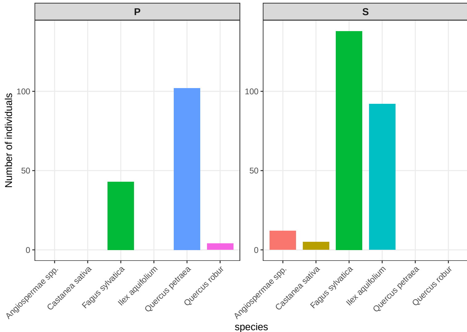
Number of individuals per sp and canopy layer on CHS 35
