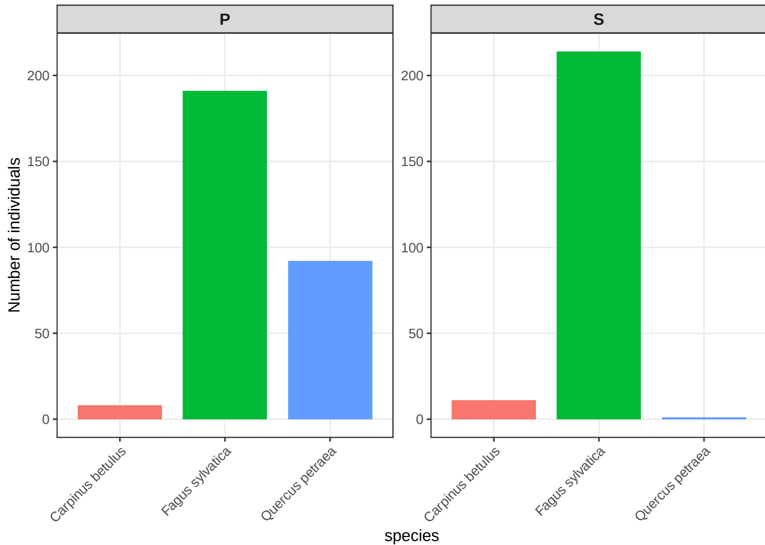
Number of individuals per sp and canopy layer on CHS 27
