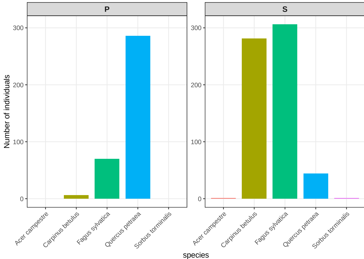
Number of individuals per sp and canopy layer on CHS 58
