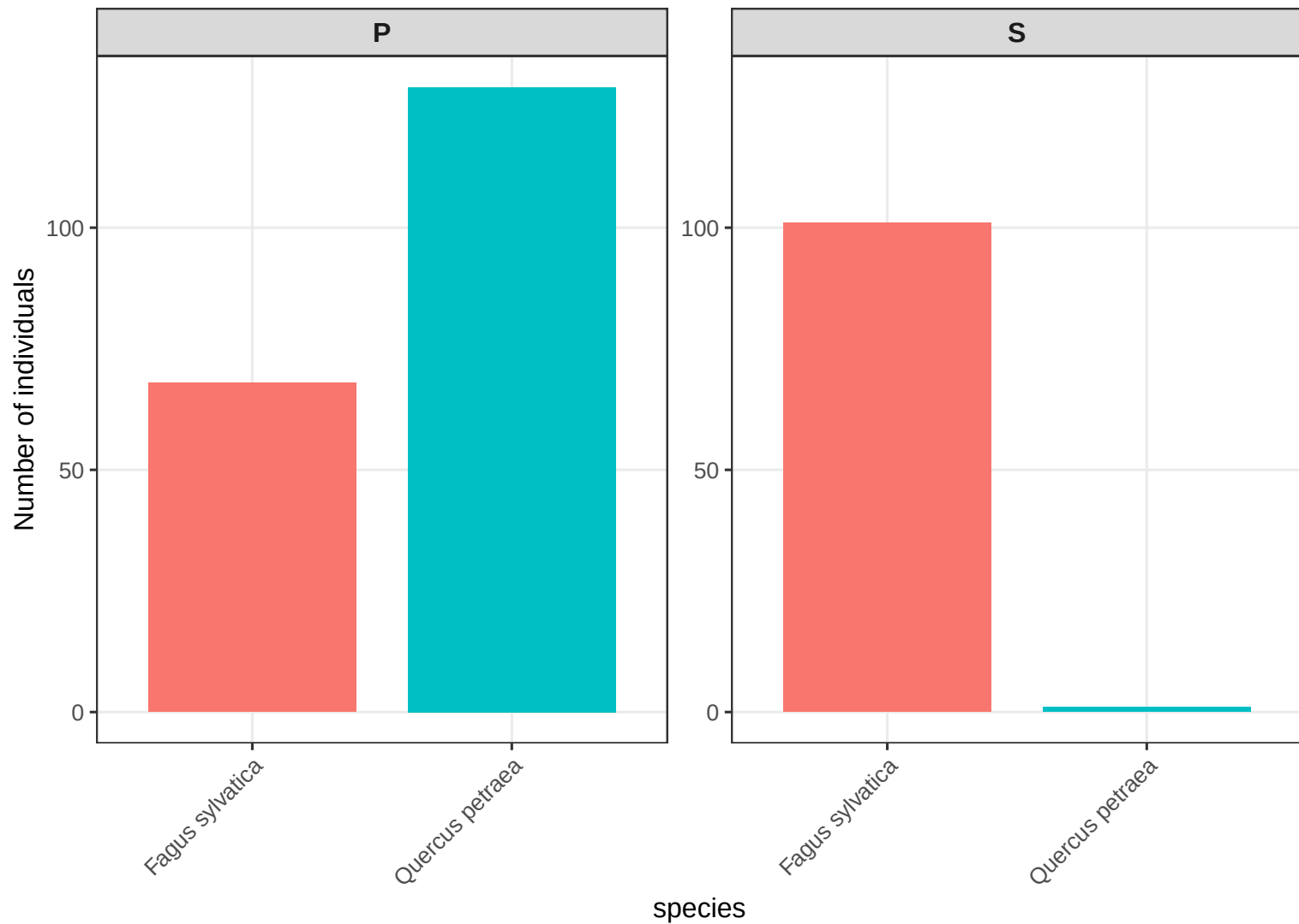
Number of individuals per sp and canopy layer on CHS 57b
