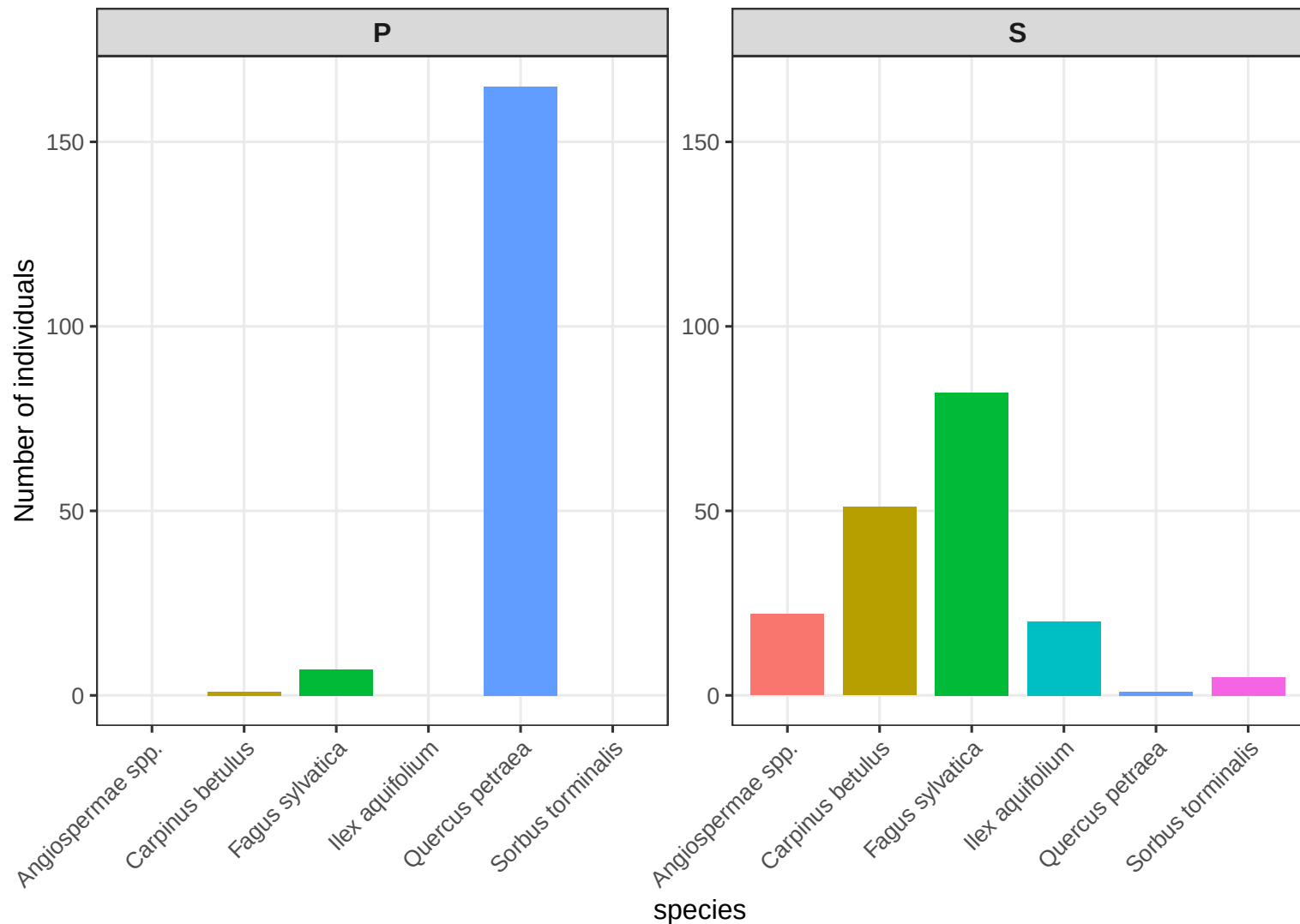
Number of individuals per sp and canopy layer on CHS 41
