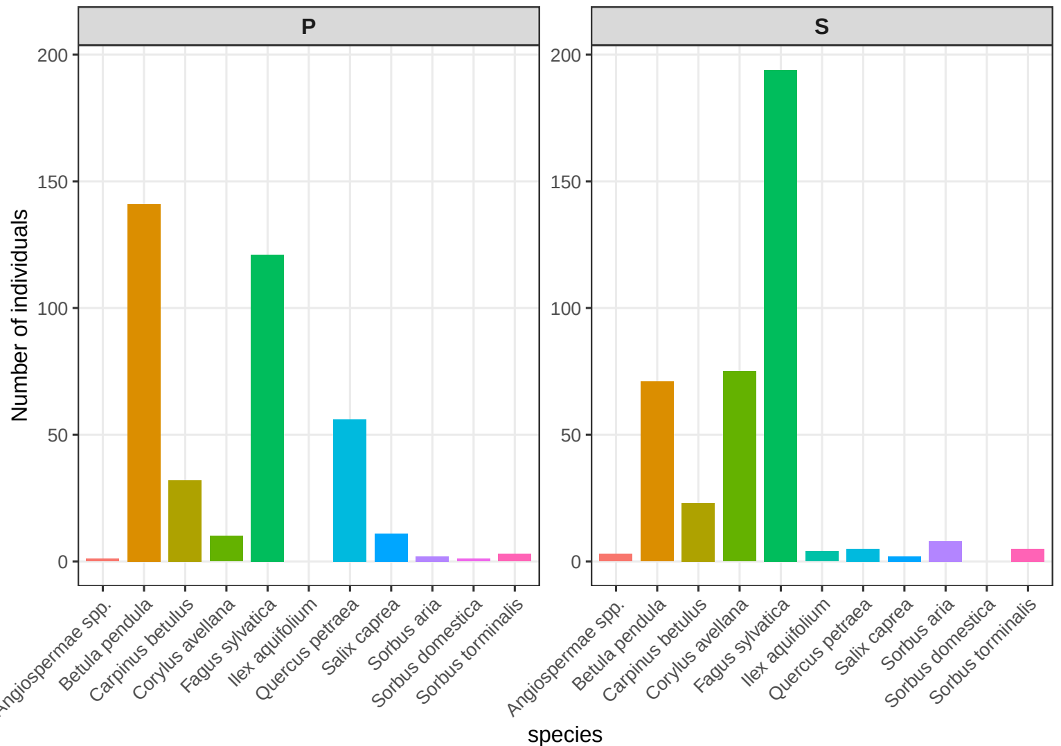
Number of individuals per sp and canopy layer on CHS 51
