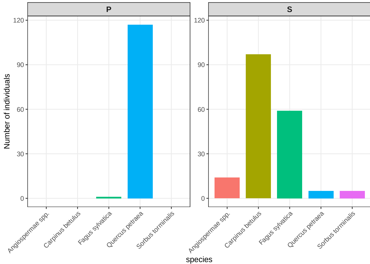
Number of individuals per sp and canopy layer on CHS 81
