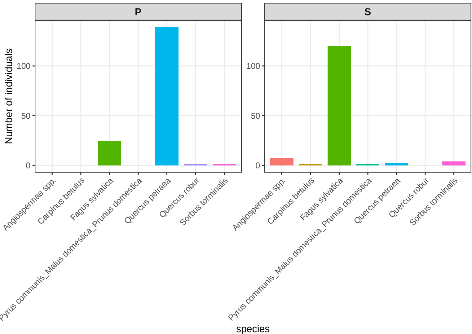
Number of individuals per sp and canopy layer on CHS 18
