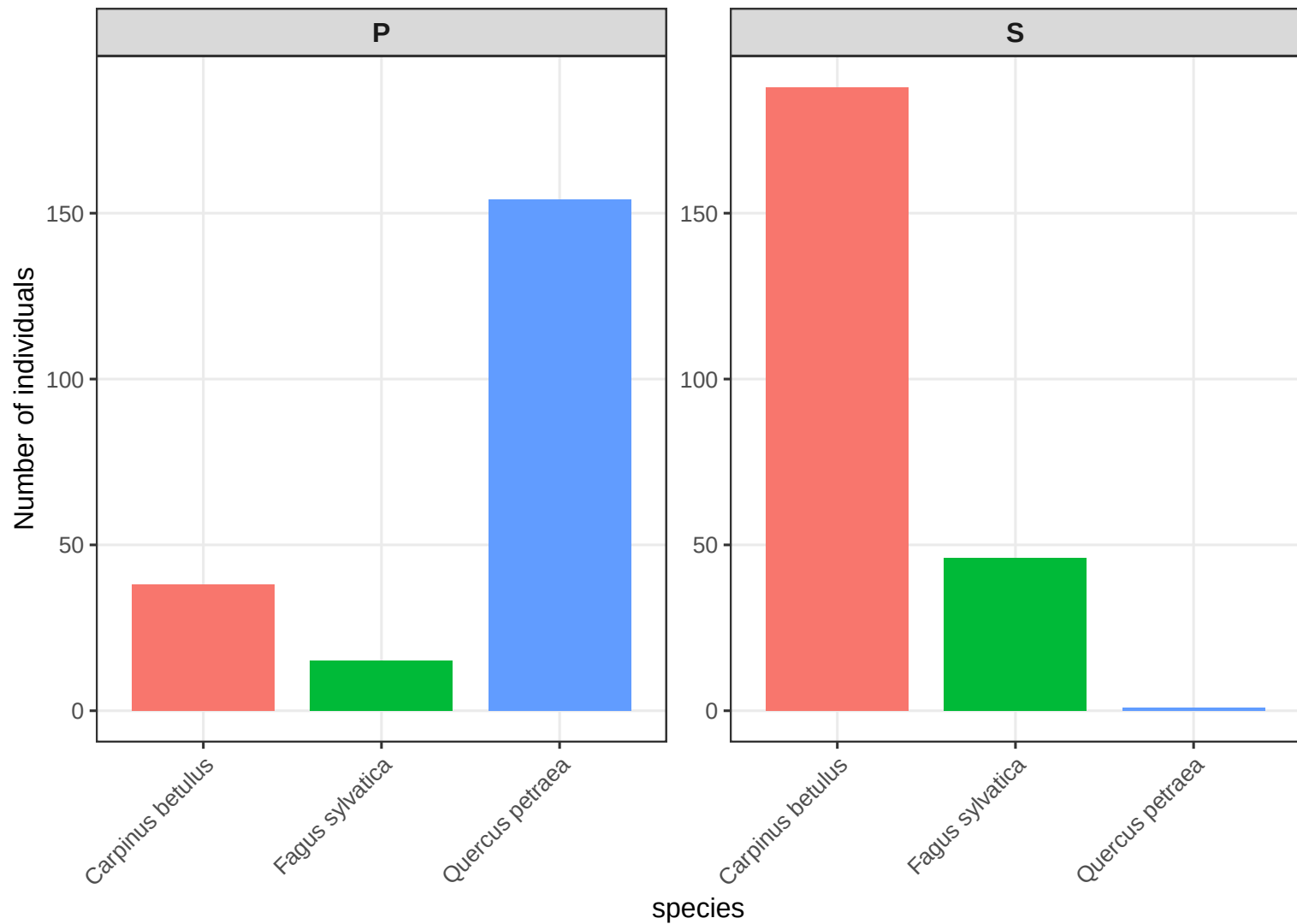
Number of individuals per sp and canopy layer on CHS 01
