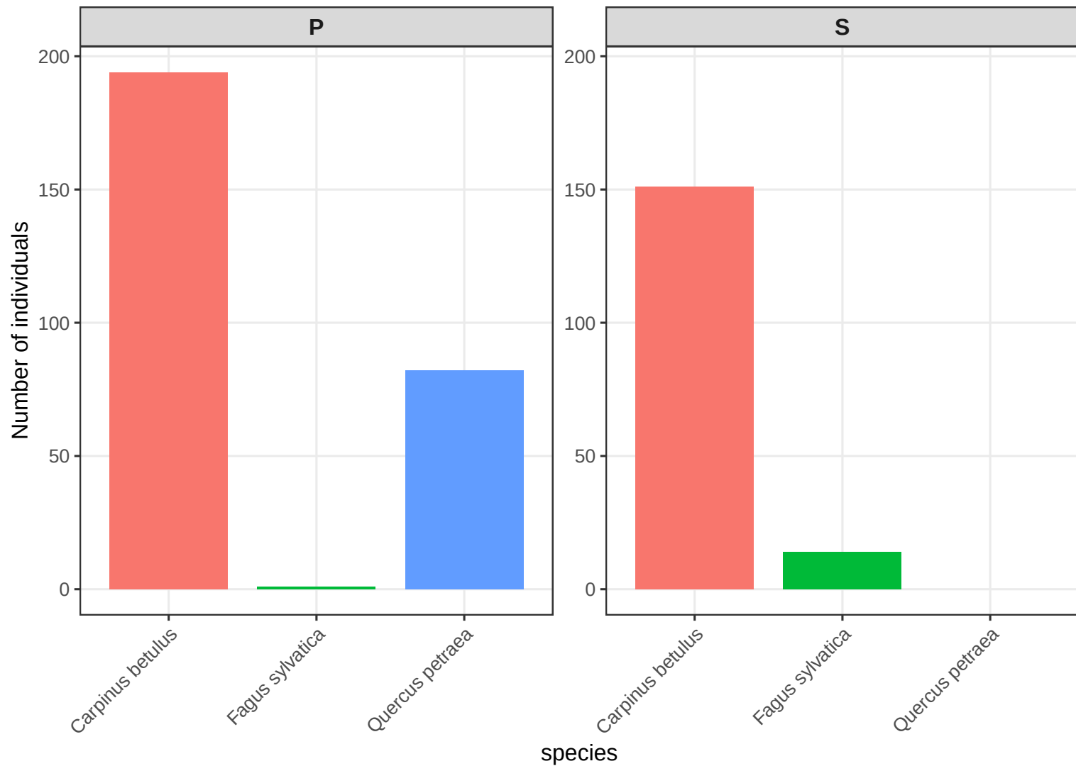
Number of individuals per sp and canopy layer on CHS 88
