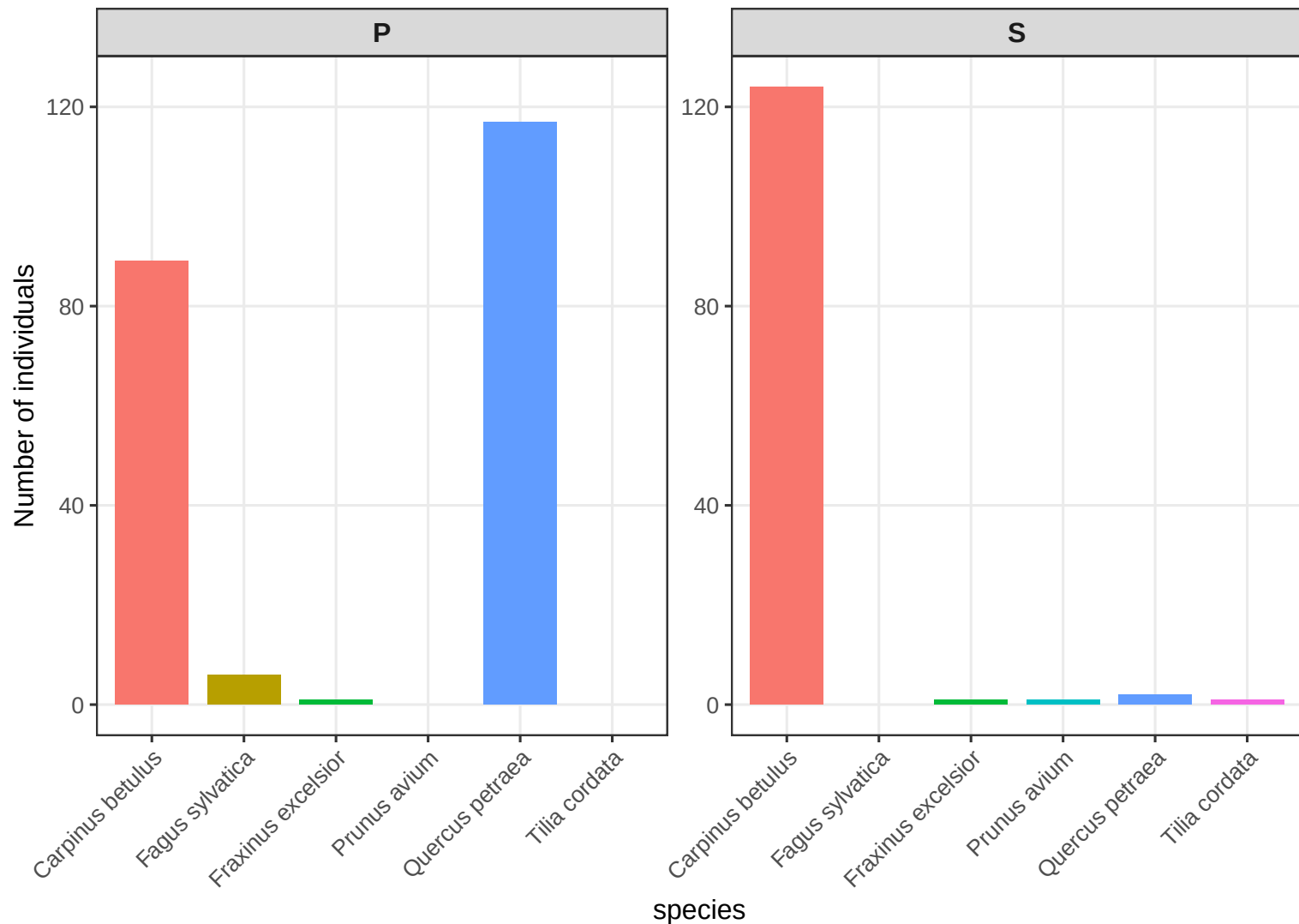
Number of individuals per sp and canopy layer on CHS 60
