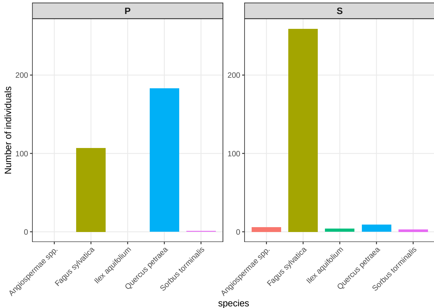
Number of individuals per sp and canopy layer on CHS 72
