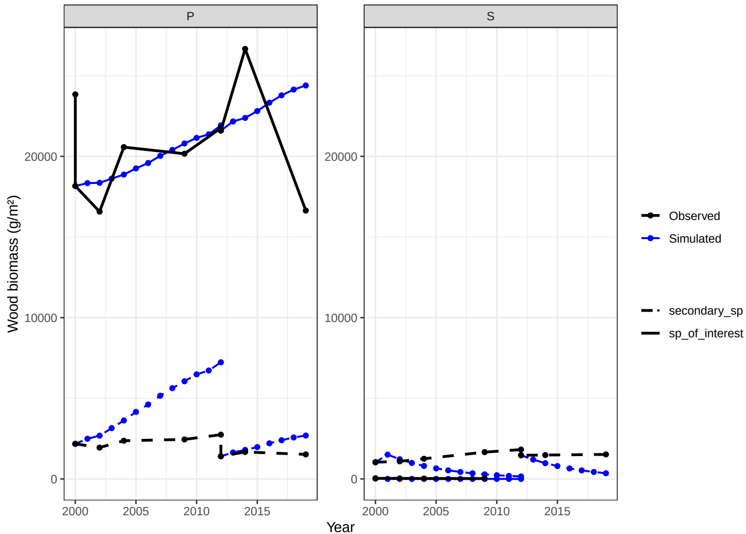
Site CHS21 – wood biomass obs vs simulated
