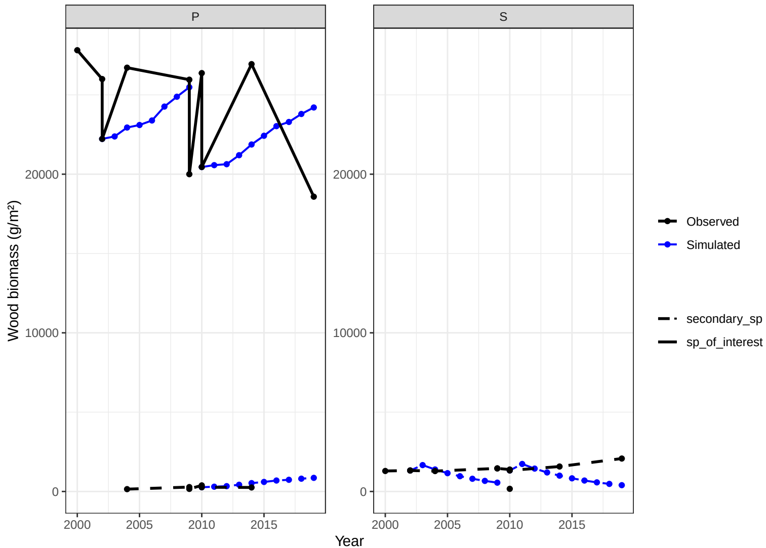
Site CHS41 – wood biomass obs vs simulated
