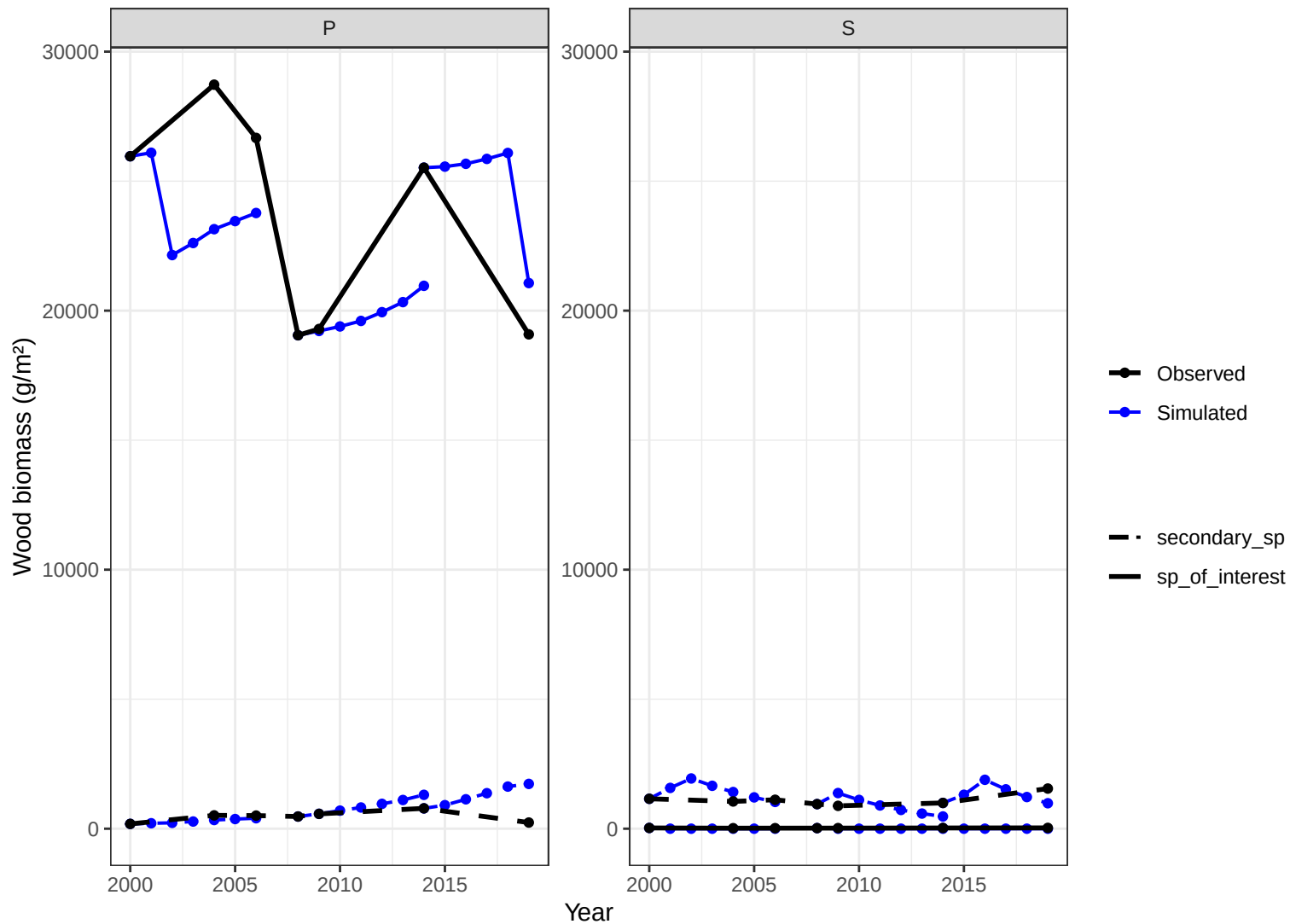
Site CHS18 – wood biomass obs vs simulated
