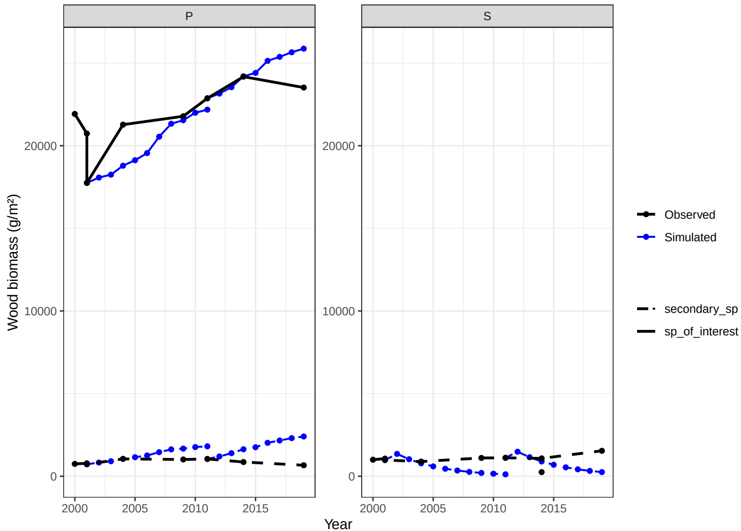
Site CHS01 – wood biomass obs vs simulated
