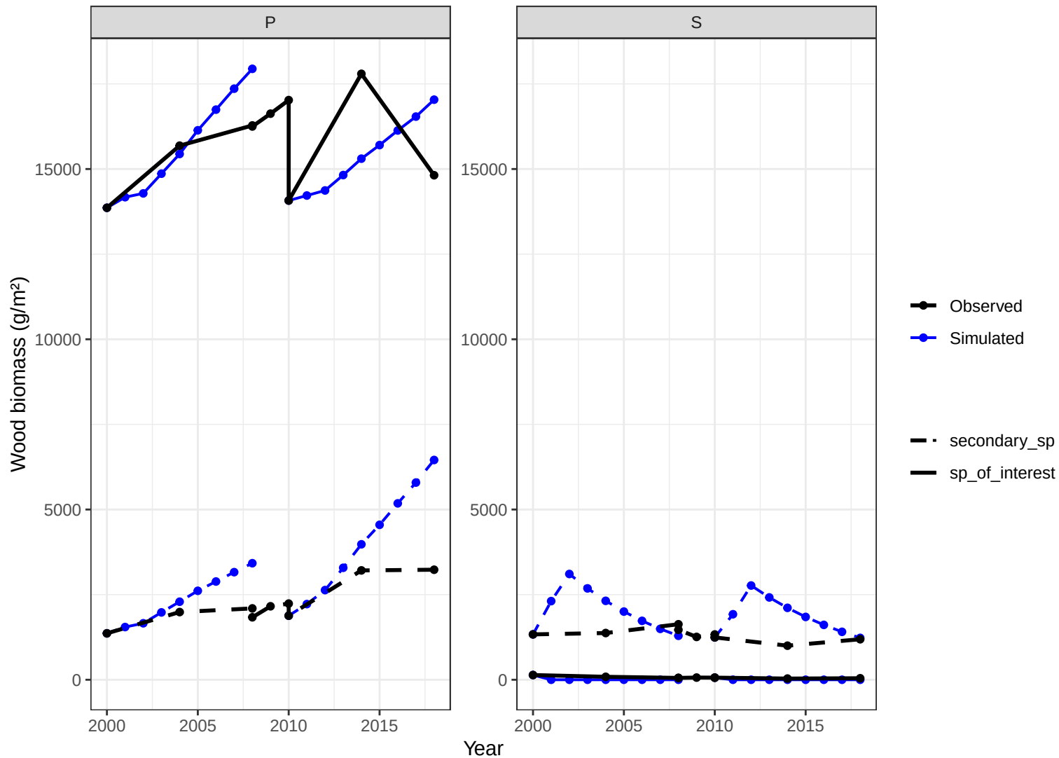
Site CHS10 – wood biomass obs vs simulated
