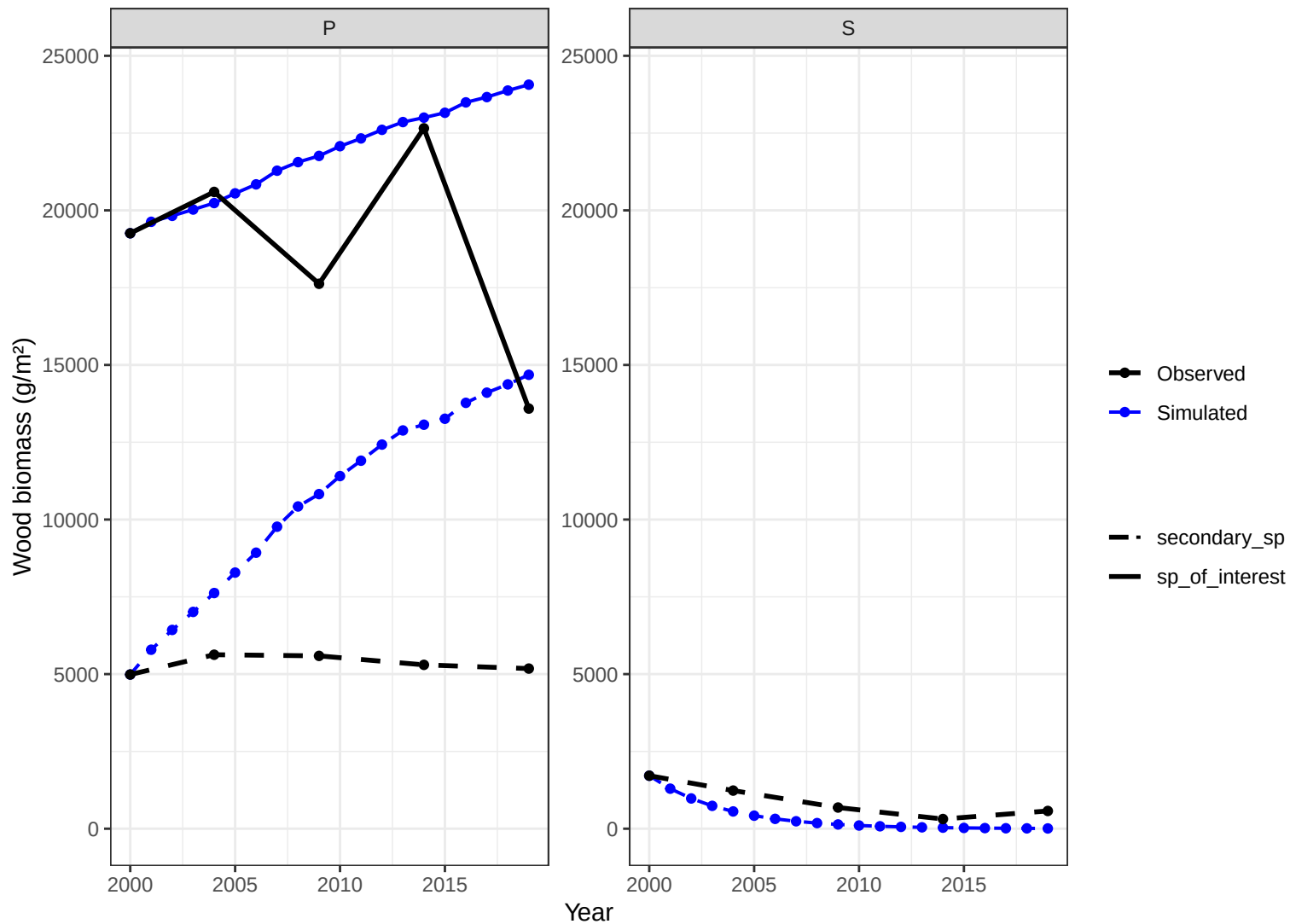
Site CHS88 – wood biomass obs vs simulated
