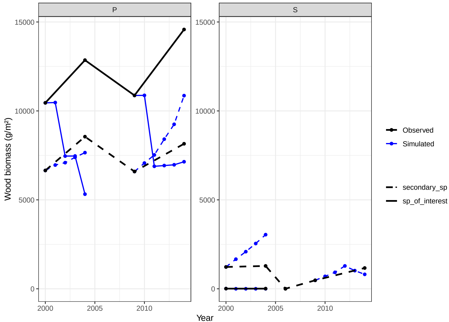
Site CHS27 – wood biomass obs vs simulated
