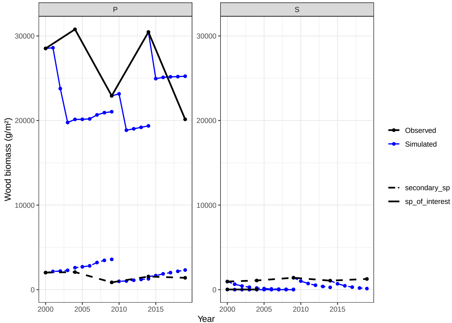
Site CHS03 – wood biomass obs vs simulated
