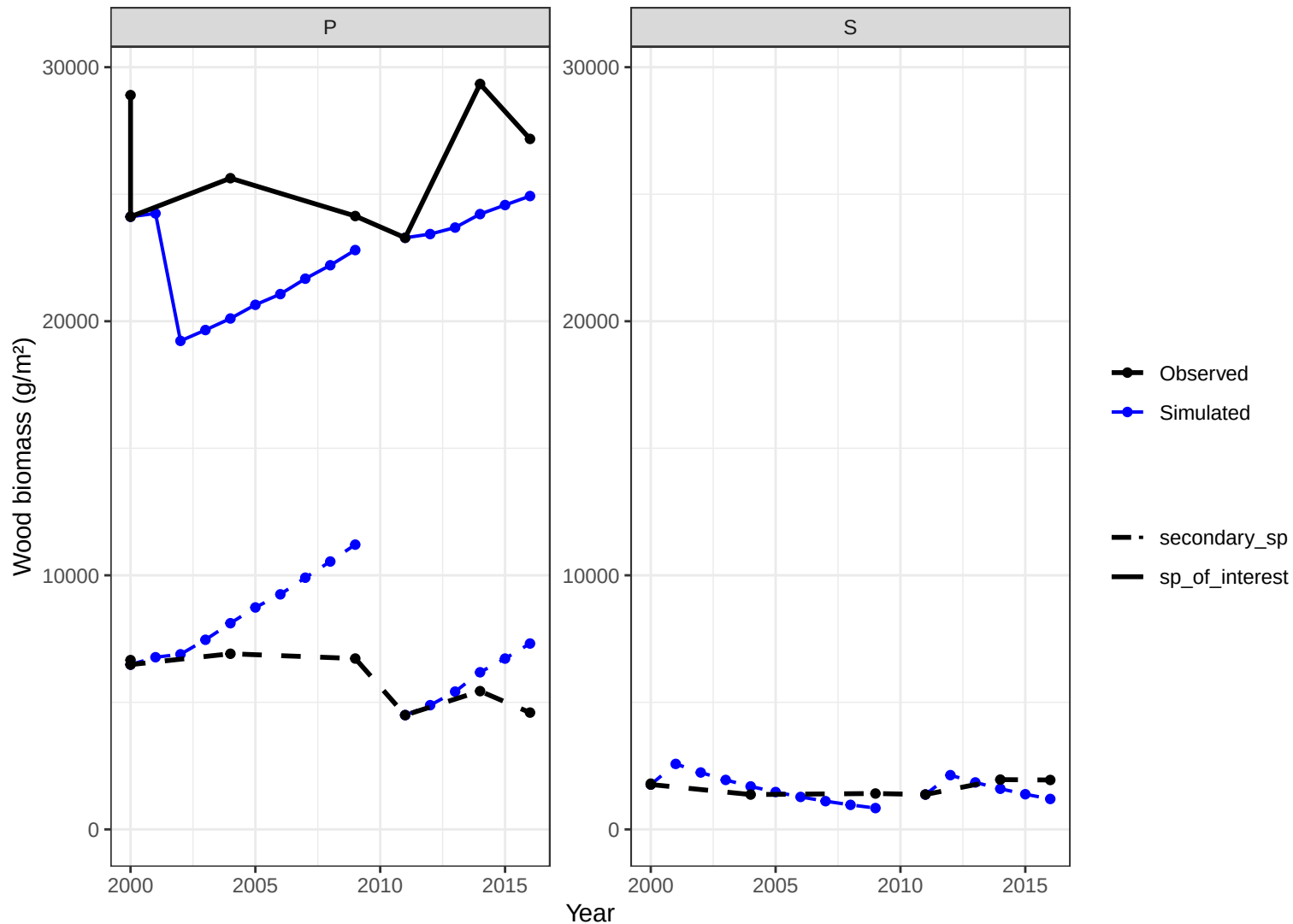
Site CHS35 – wood biomass obs vs simulated
