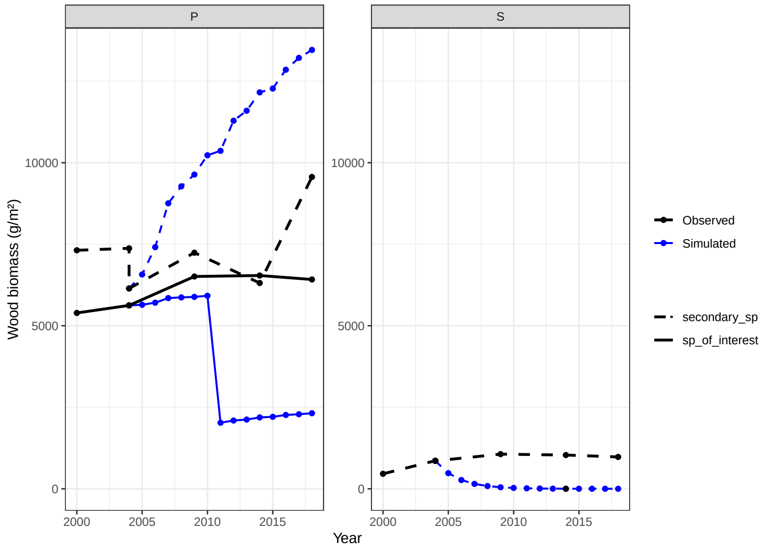
Site CHS68 – wood biomass obs vs simulated
