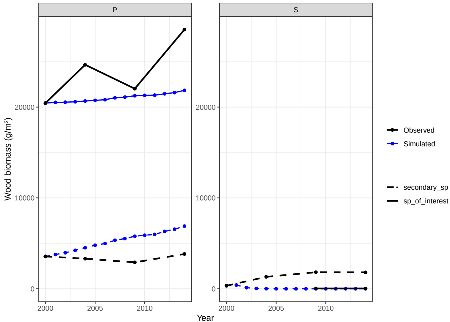
Site CHS60 – wood biomass obs vs simulated
