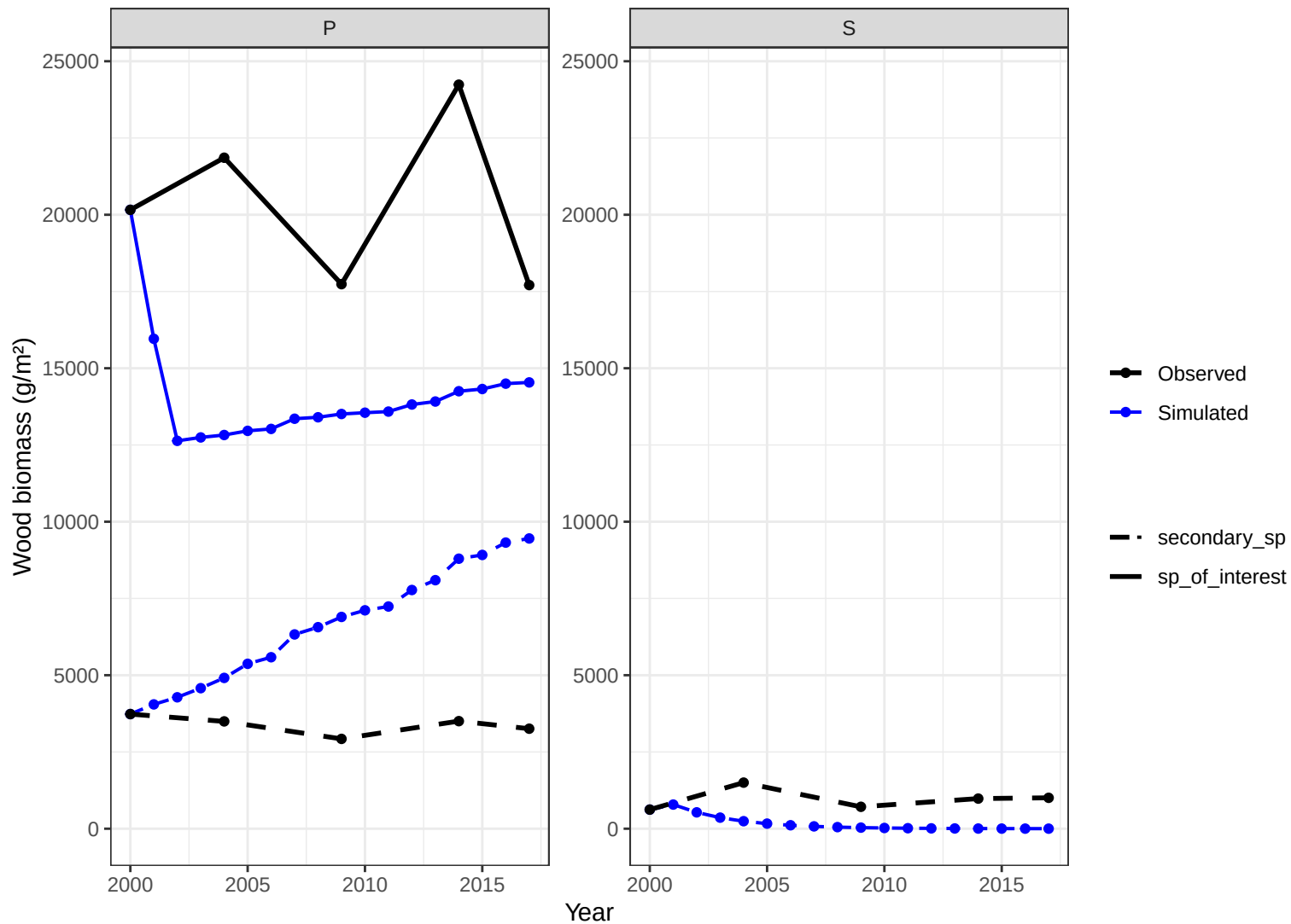
Site CHS61 – wood biomass obs vs simulated
