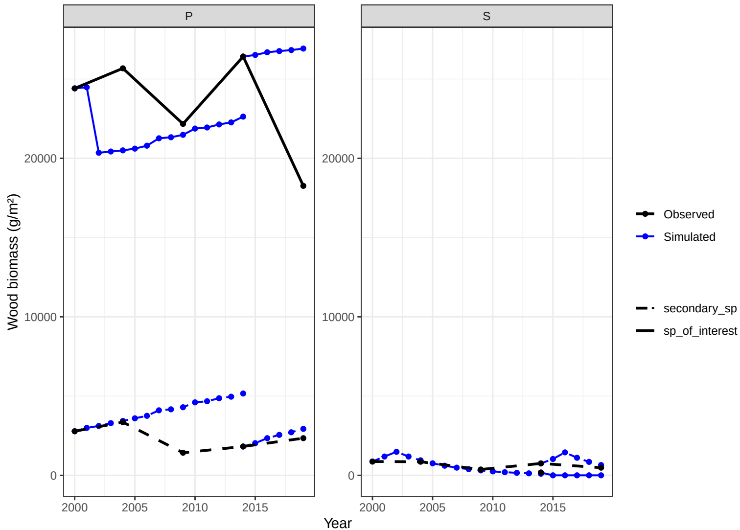
Site CHS57b – wood biomass obs vs simulated
