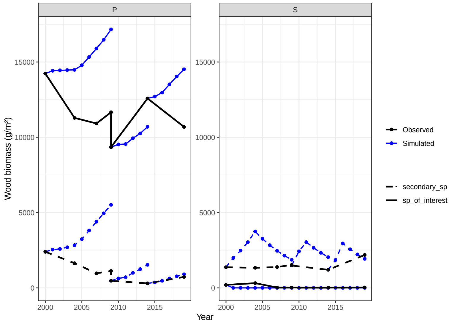
Site CHS58 – wood biomass obs vs simulated
