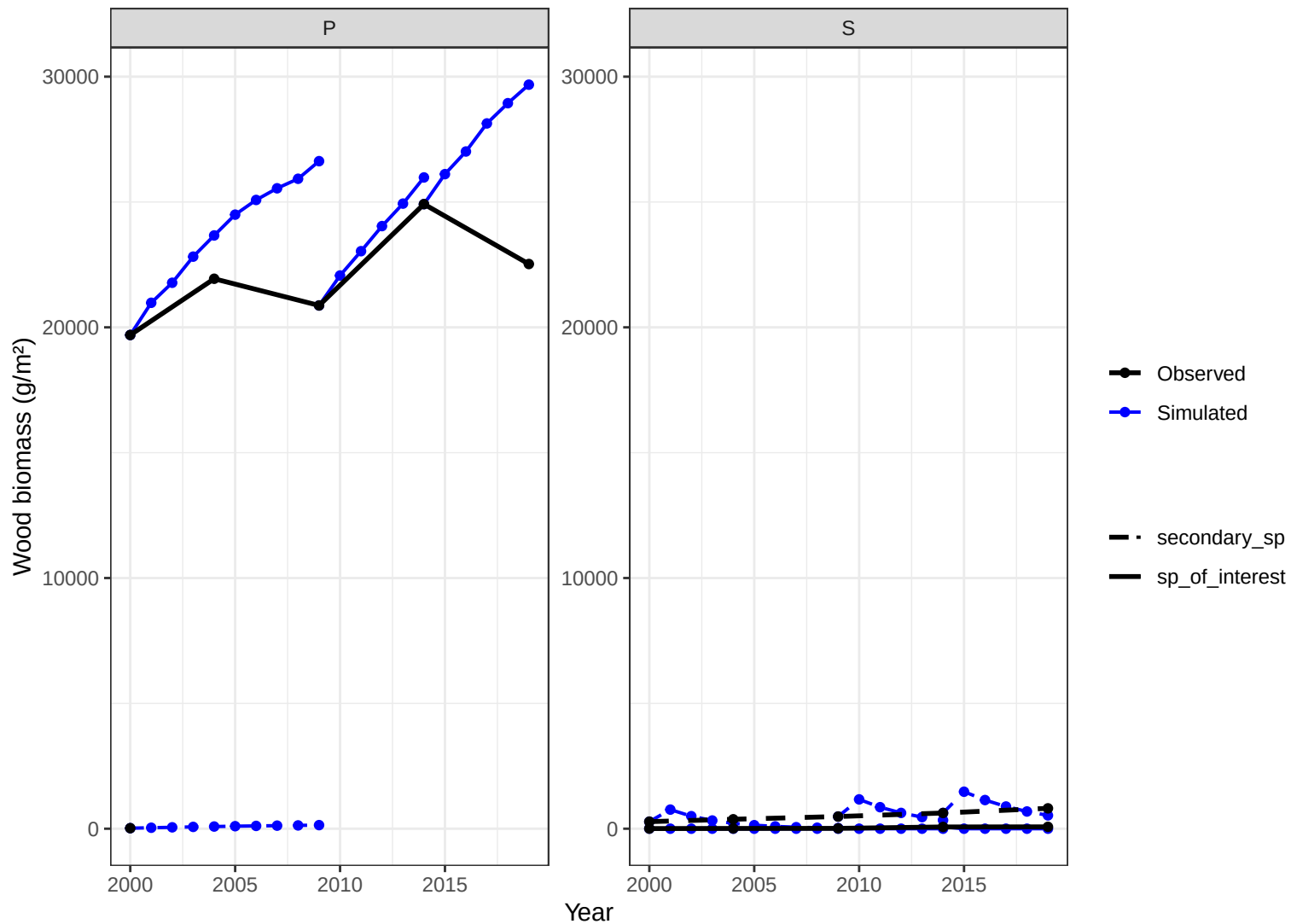
Site CHS81 – wood biomass obs vs simulated
