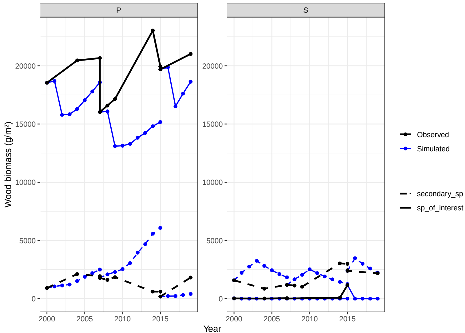
Site CHS72 – wood biomass obs vs simulated
