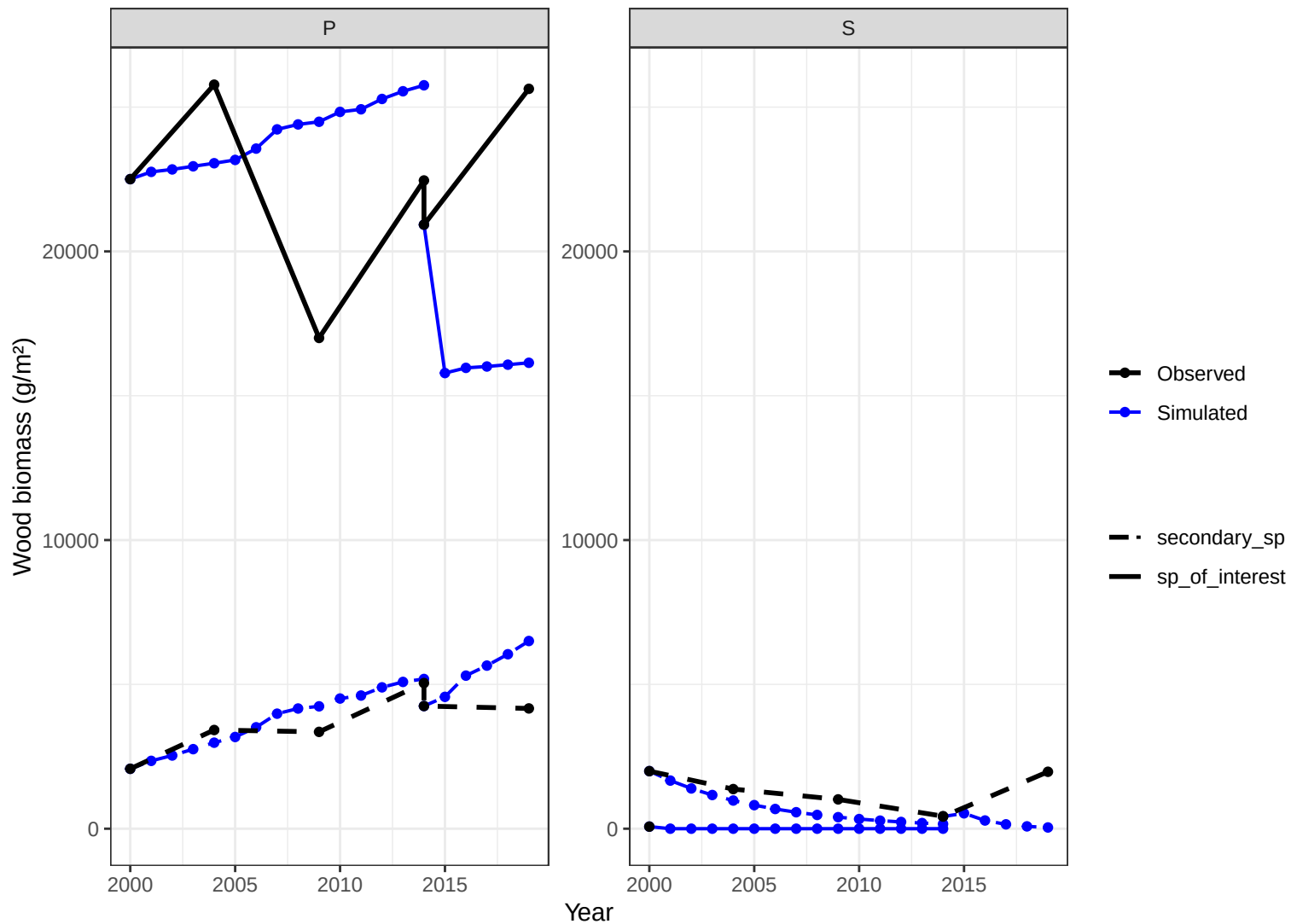
Site CHS57a – wood biomass obs vs simulated
