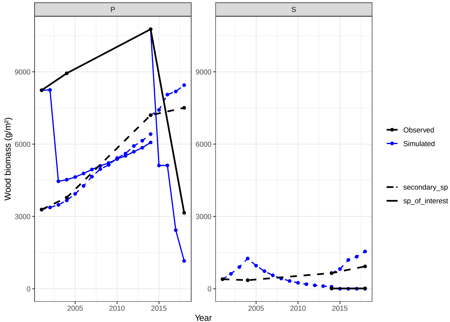
Site CHS51 – wood biomass obs vs simulated
