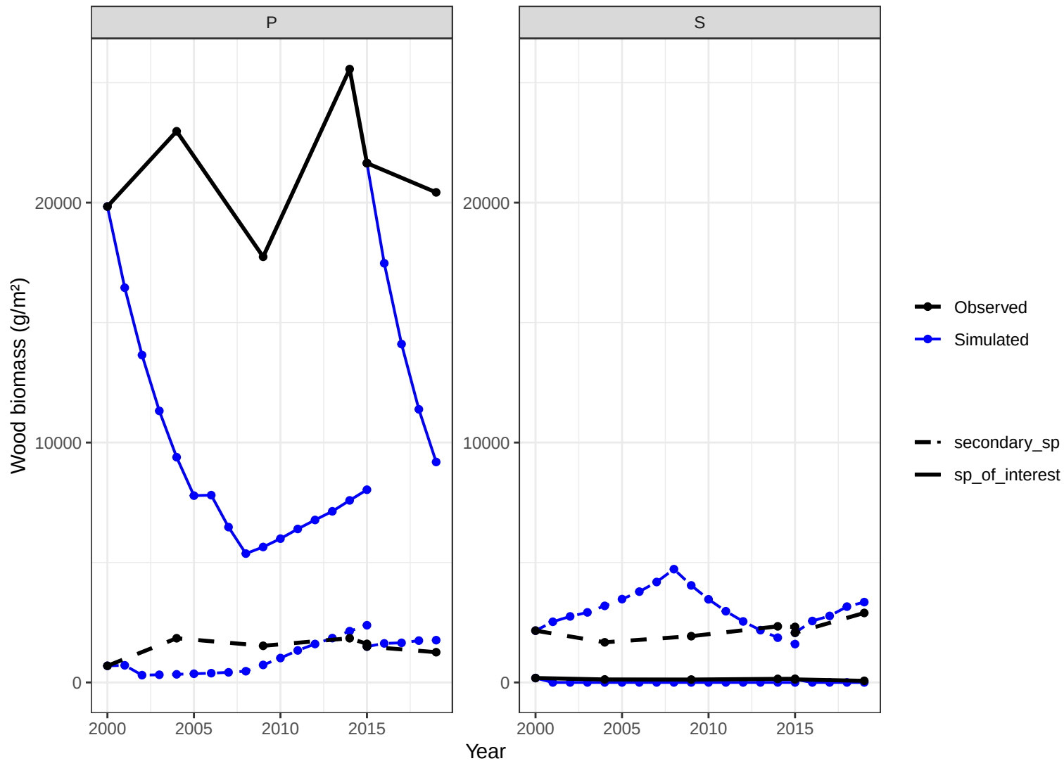
Site CHS86 – wood biomass obs vs simulated
