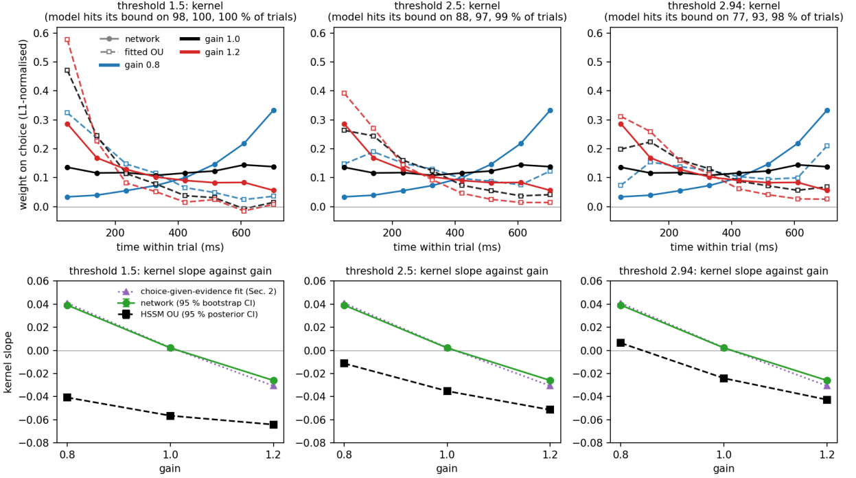
Figure 3. Kernel check at thresholds 1.5, 2.5 and 2.94. Top: kernels, network (solid) vs the fitted OU with its fitted bound driven by the same evidence (dashed). Bottom: kernel slope against gain; network with 95 % bootstrap interval over trials, HSSM OU with 95 % posterior interval over 40 draws, and the choice-given-evidence fit of Section 2 for reference. Both intervals are about \pm 0.001 , smaller than the markers.
