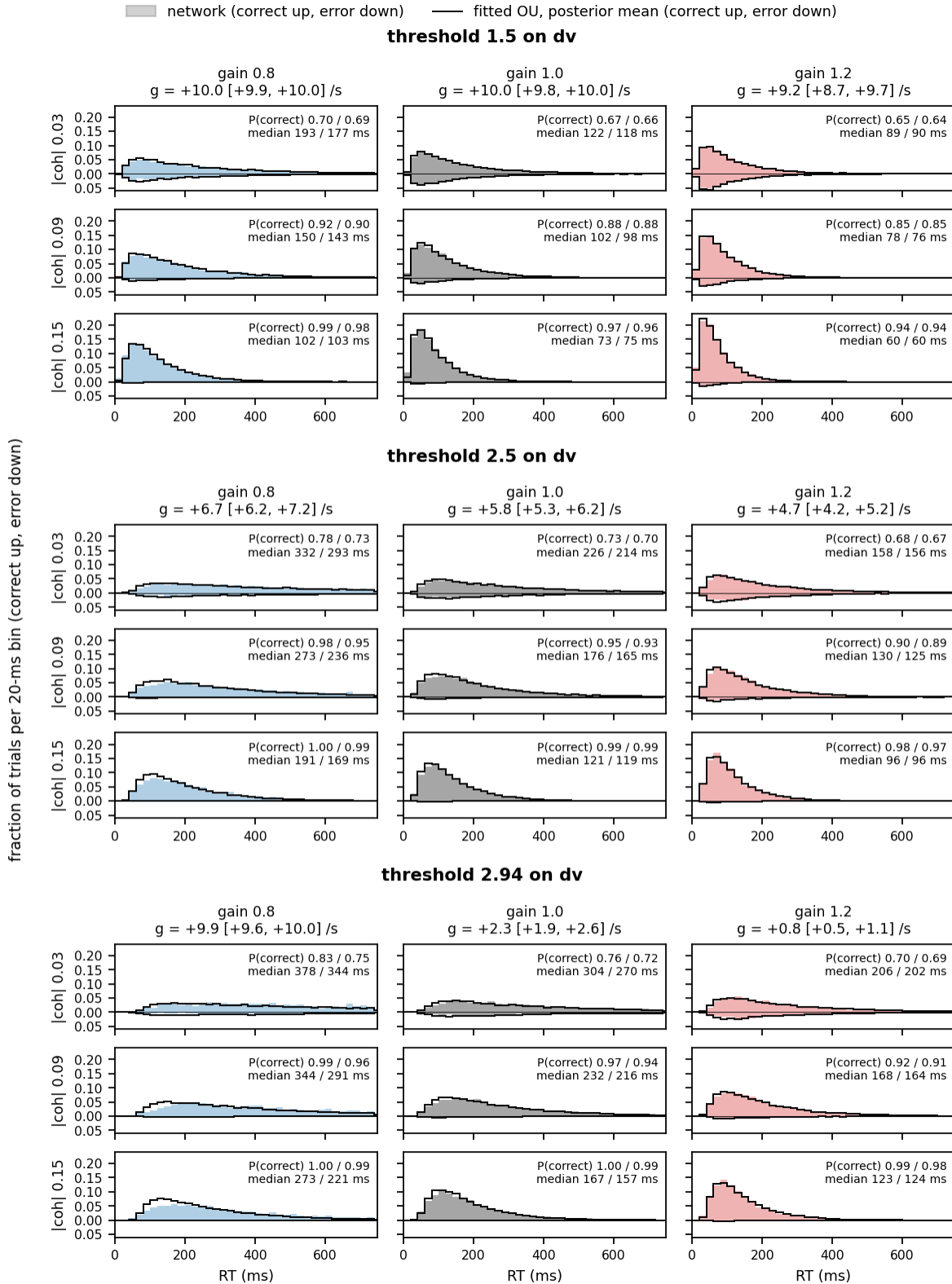
Figure 2. RT posterior predictive by threshold (blocks), [coherence] (rows) and gain (columns). Fraction of trials per 20-ms bin, correct up and errors down (the two sum to one), on the same scale in every panel; network (filled) vs fitted OU at its posterior mean (line). Column titles: native g with 95 % posterior interval; insets: accuracy and median RT, network / model. At 1.5 the fit is close everywhere; at 2.5 and 2.94 it misses the leaky network's slow, flat RT distribution at every coherence, while gain 1.2 stays well described.
