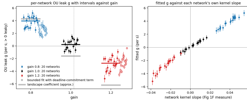
Figure 4. Left: fitted g per network with 94 % HDIs (filled), pooled fit (bars), bounded fit with the deadline-commitment term (open squares), landscape drift coefficient (gray), kernel zero crossing of Fig 1F at gain 1.016 (dotted). Right: g against each network's own kernel slope, r = 0.996 .
