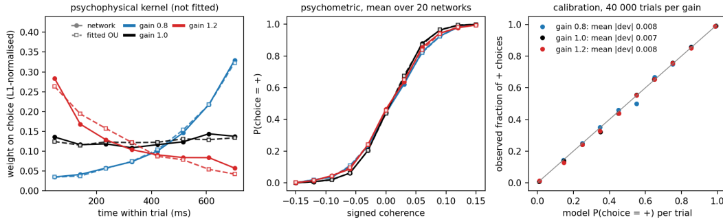
Figure 5. Posterior predictive. Left: the fit reproduces the psychophysical kernel it was not fitted to (slopes +0.041 / +0.002 / -0.031 vs network +0.039 / +0.002 / -0.026 ). Middle: P(\text{choice}) by signed coherence, within 0.015 everywhere. Right: per-trial predicted probability against observed choice fraction.
