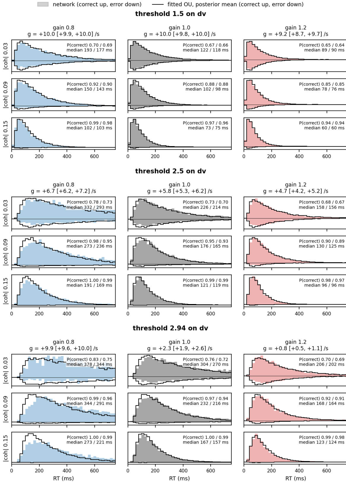
Figure 2. RT posterior predictive by threshold (blocks), [coherence] (rows) and gain (columns). Correct trials up, errors down, each normalised to sum to one; network (filled) vs fitted OU at its posterior mean (line). Column titles: native g with 95 % posterior interval; insets: accuracy and median RT, network / model. At 1.5 the fit is close everywhere; at 2.5 and 2.94 it misses the leaky network's slow, flat RT distribution at every coherence, while gain 1.2 stays well described.
