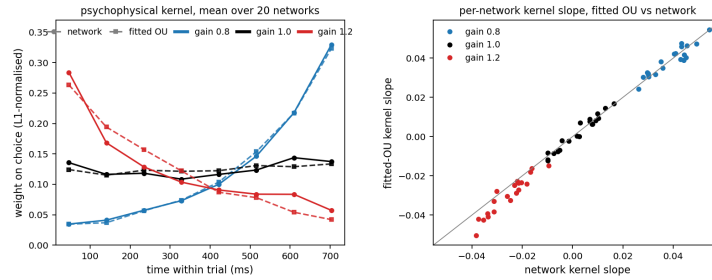
Figure 3. Track B. Left: psychophysical kernels of the networks (solid) and of the fitted OU driven by the same evidence streams (dashed), averaged over the twenty networks. Right: kernel slope of the fitted model against that of the network, one point per network and gain.
