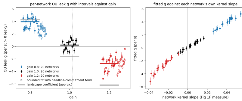
Figure 2. Track B. Left: fitted OU leak g per network with 94 percent intervals against gain (filled, unbounded fit), the bounded fit with the deadline-commitment term (open squares, gains 0.8 and 1.2), pooled fits (coloured bars), landscape coefficients (gray bars) and the kernel zero crossing of Figure 1F at gain 1.016 (dotted). Right: the same estimates against each network's own kernel slope. Positive g is leaky.
