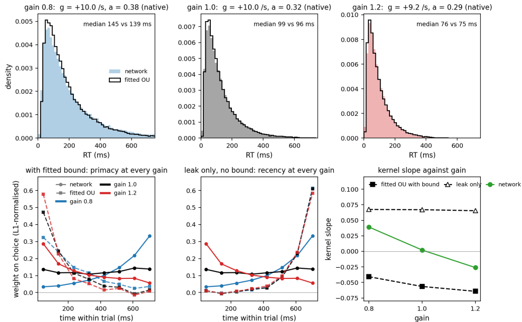
Figure 1. Track A. Top: RT distributions of the twenty networks (filled) and of the HSSM-fitted OU at its pooled posterior mean (line), all coherences, constant bound 1.5. Bottom: psychophysical kernels of the networks (solid) and of the fitted OU driven by the same evidence streams (dashed), with its fitted bound (left) and without (middle); kernel slope against gain for both (right). Positive g is leaky.
