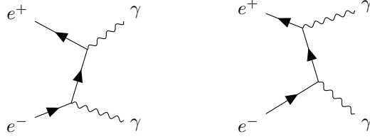
Figure 1: Figure 1: Feynman graph for the lowest order contributions to electron position annihilation [1].
