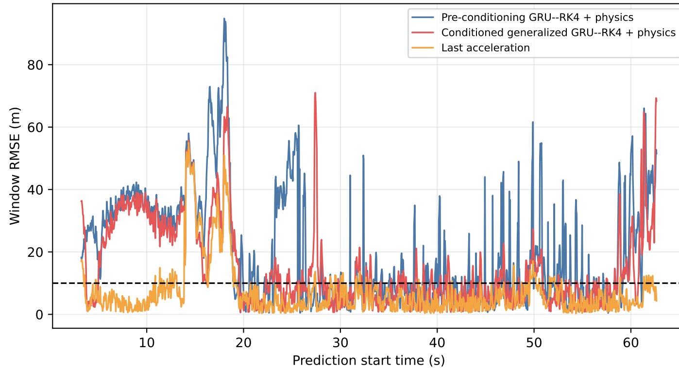
100-step Z-position error over the real flight
