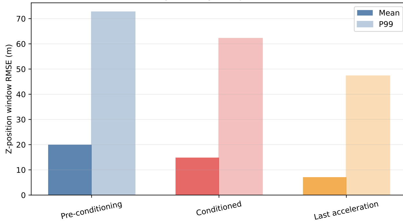
Average and high-tail position error
