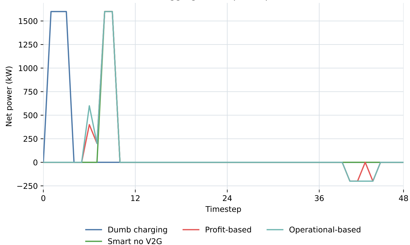
DA aggregate net power profiles
