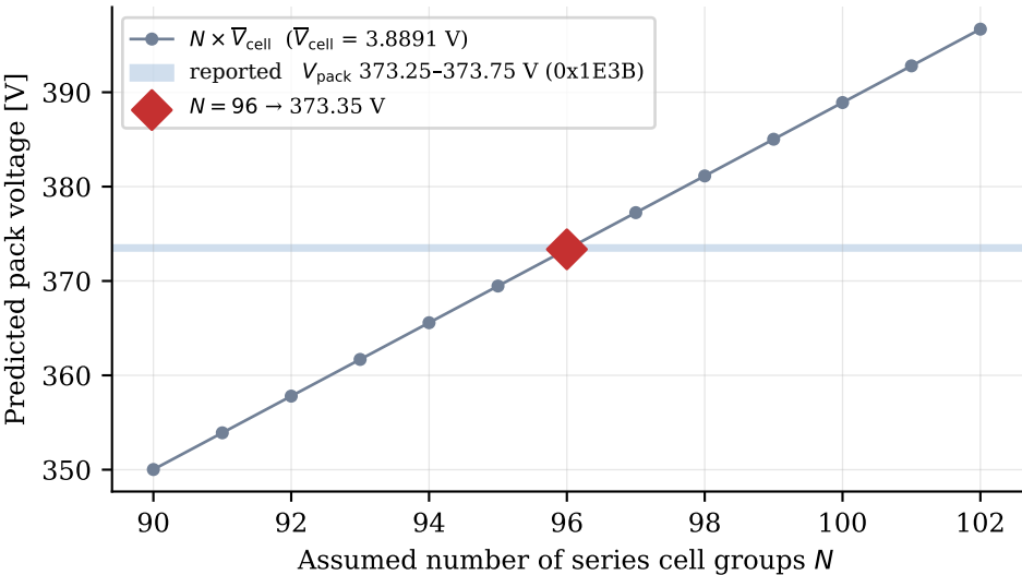
Series-count inference: only N = 96 reproduces the reported pack voltage
