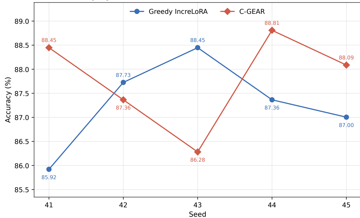
RTE Accuracy by Seed
