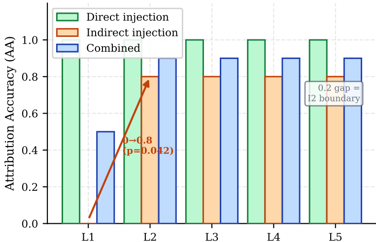
Attribution Accuracy by Level and Attack Type
