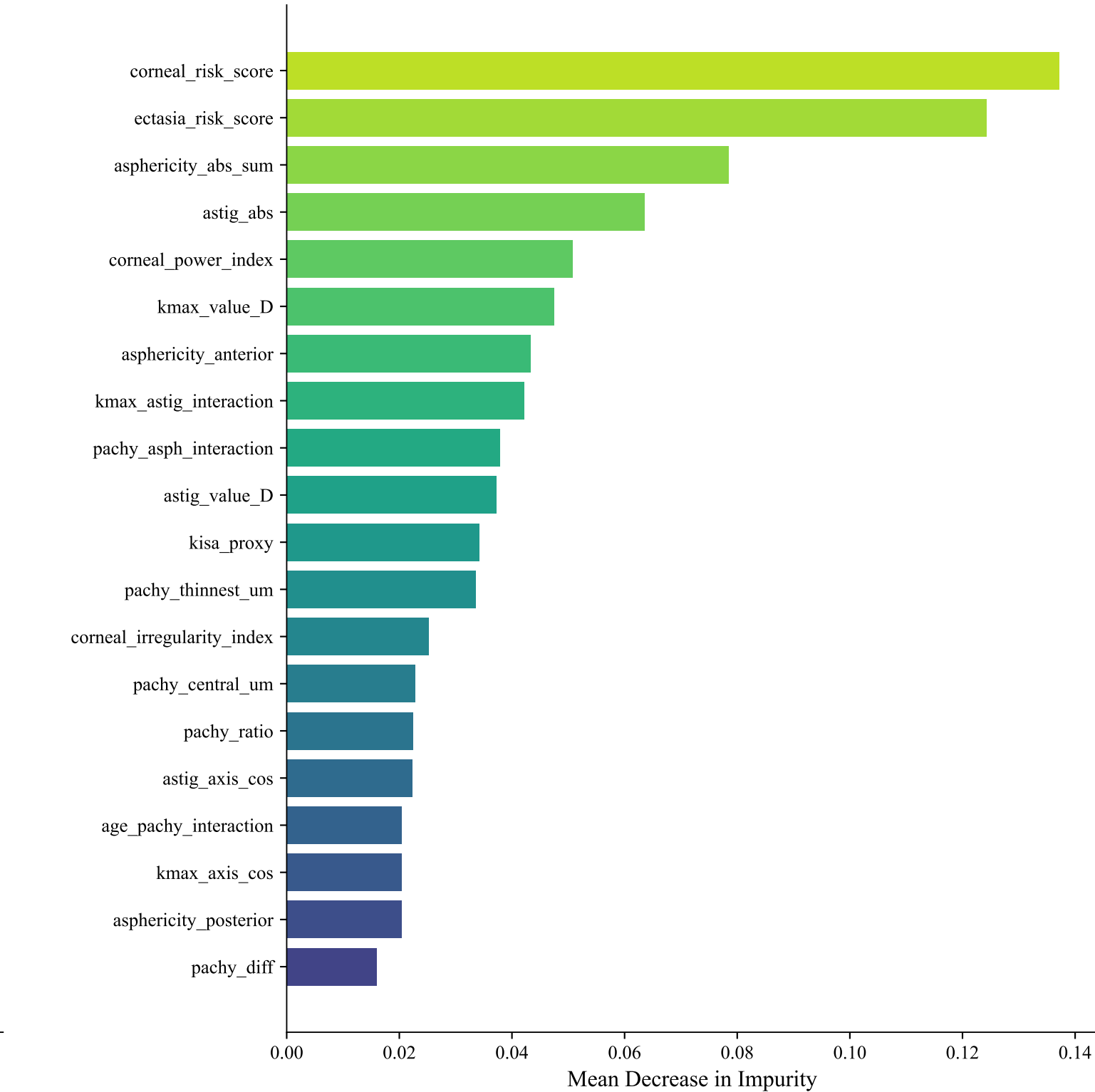
Extra Trees Feature Importance (Top 20)
