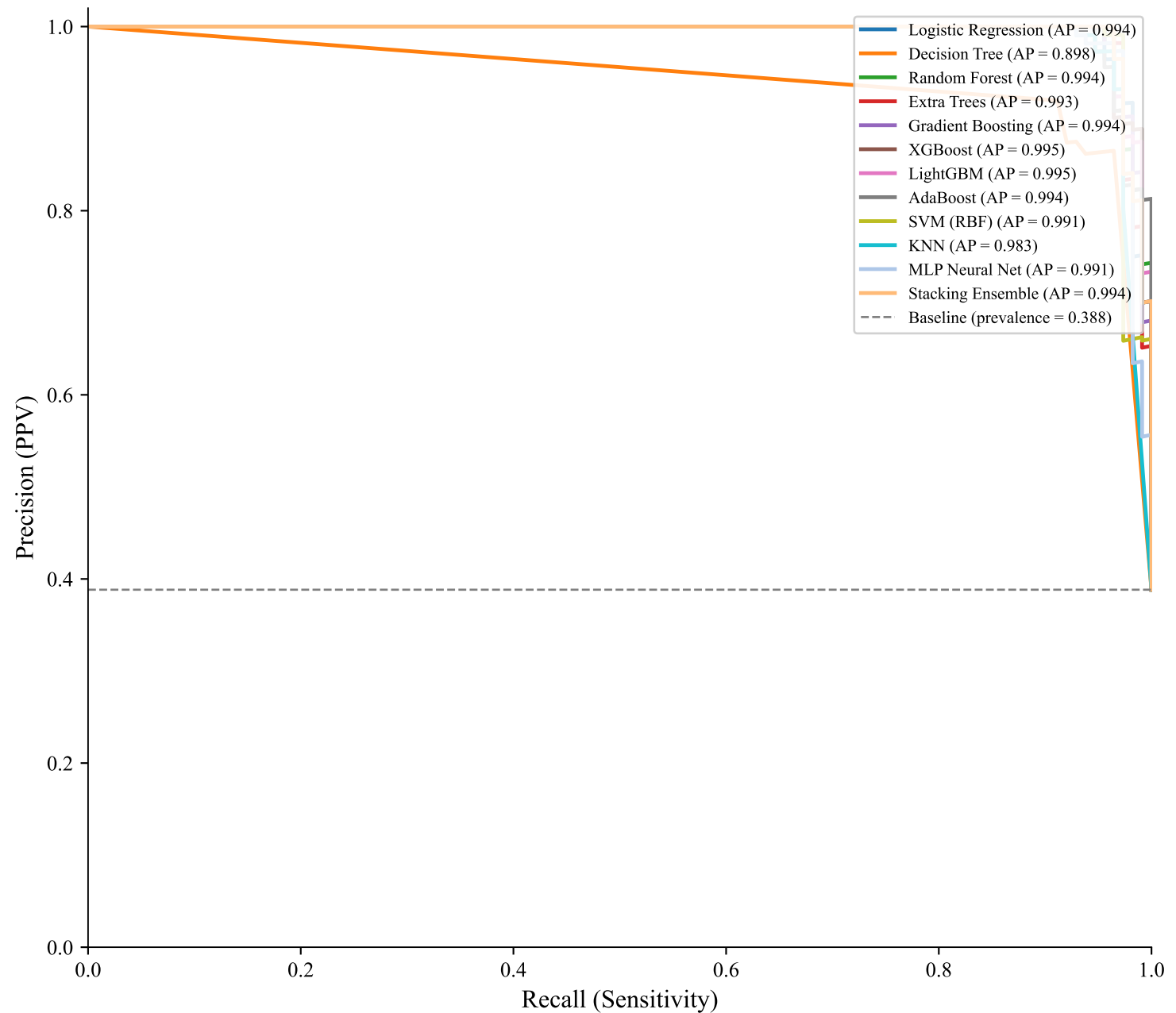
Precision-Recall Curves — All Models
