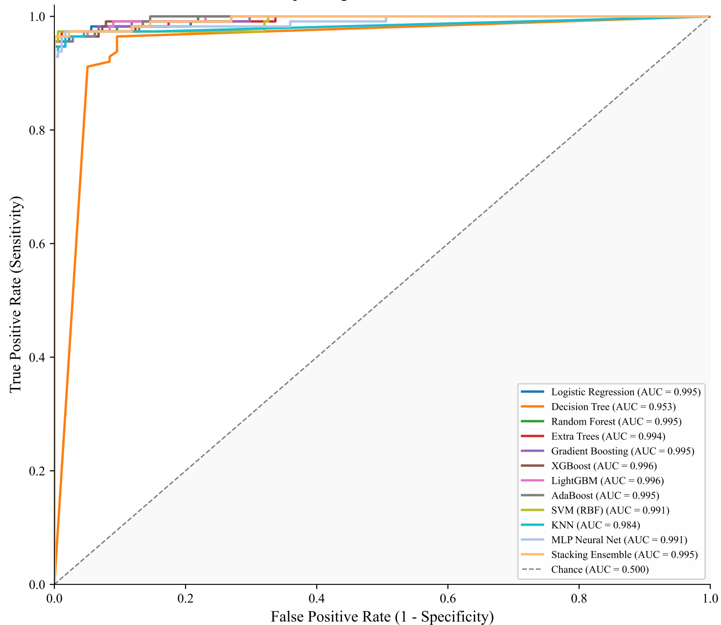
Receiver Operating Characteristic — All Models
