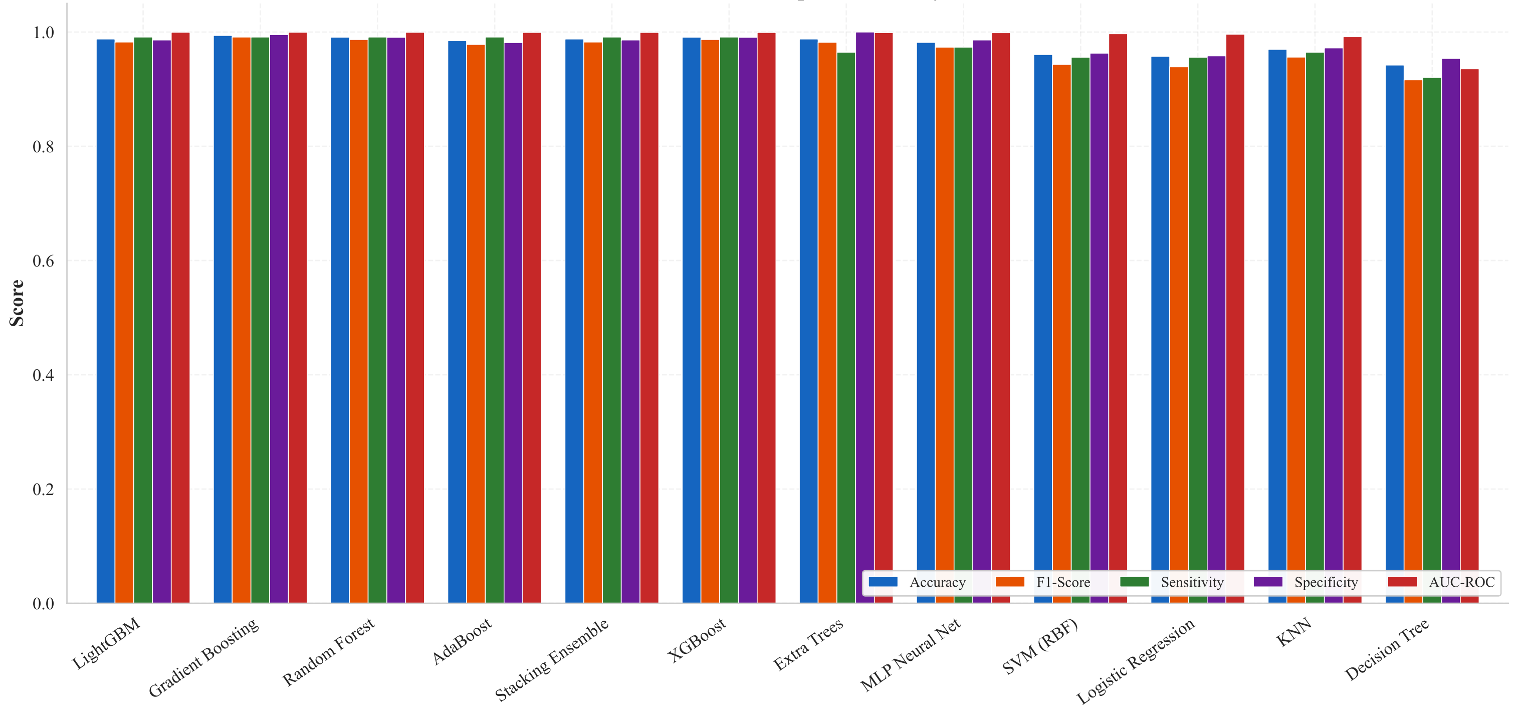
Model Performance Comparison — Key Metrics
