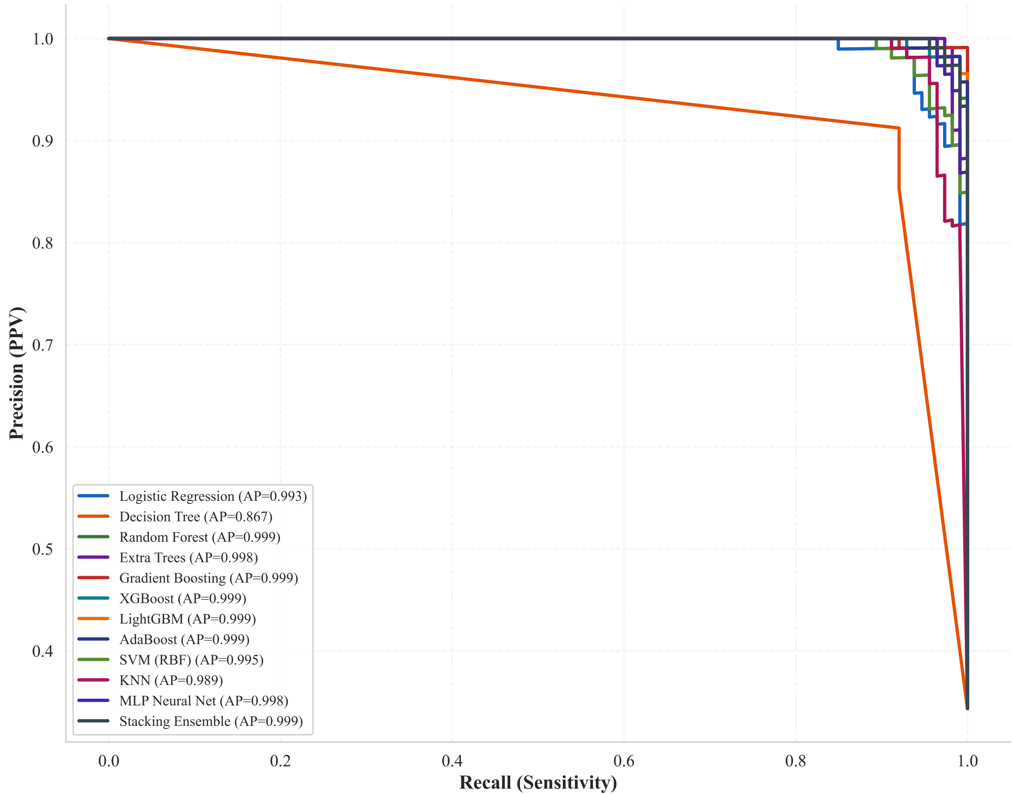
Precision–Recall Curves — All Models
