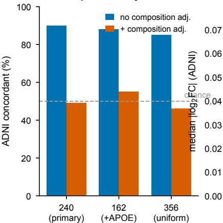
Replication collapses under composition adjustment
