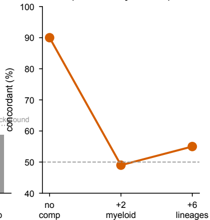
Even 2 covariates collapse it (no over-adjustment)
