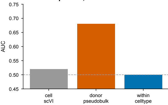
Single-cell: composition- separable, cell-intrinsic null
