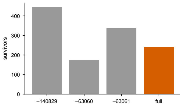
Leave-one-out meta: not single-cohort driven
