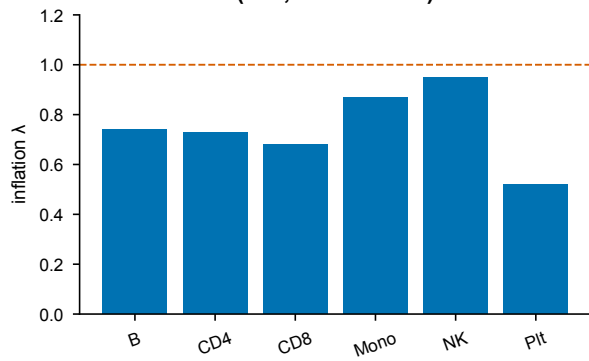
Pseudobulk calibrated ( \lambda \leq 1 , no inflation)
