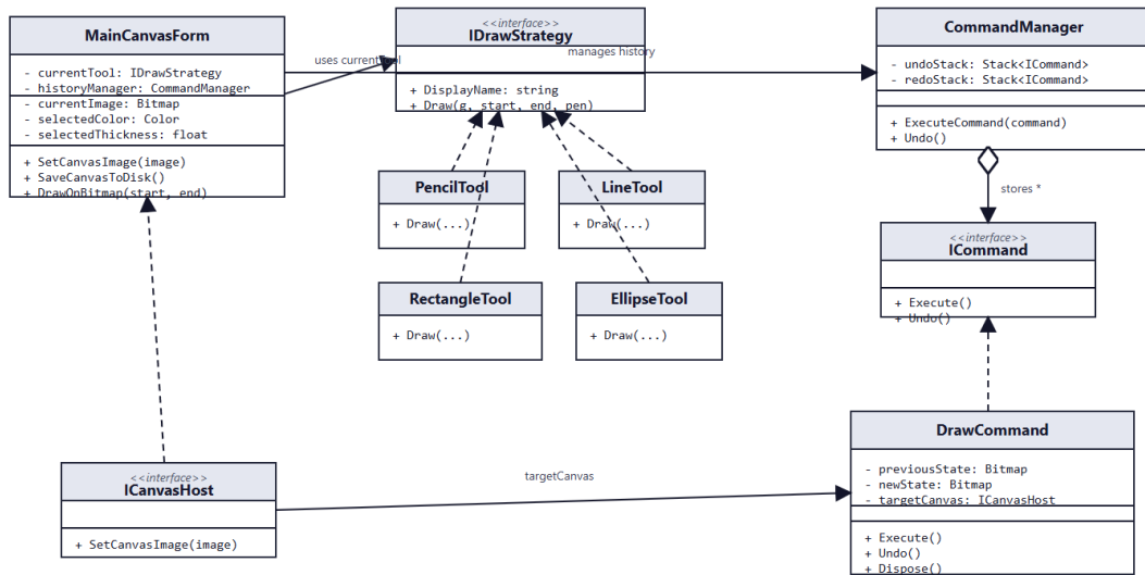
Class Diagram - Paint App
