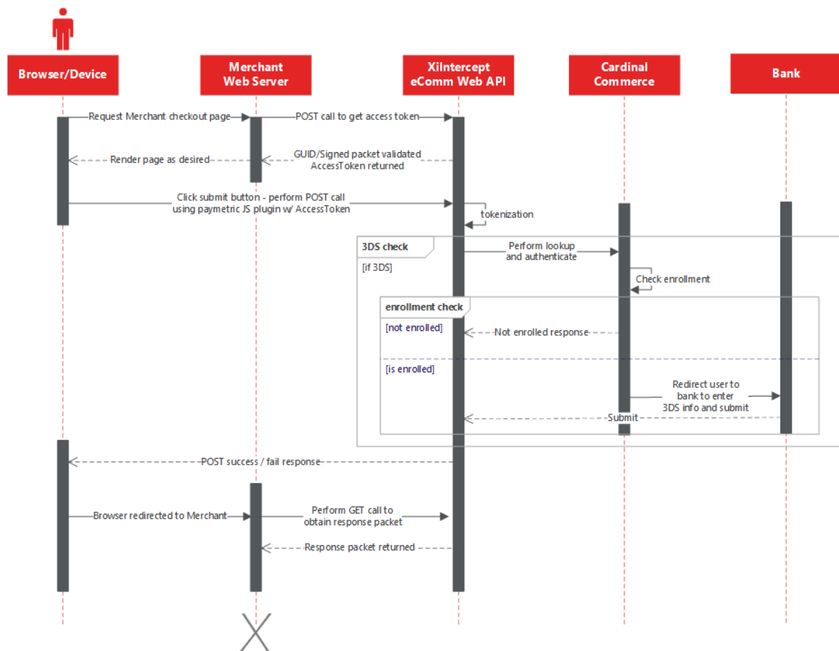
Figure 1: Form Post Integration Sequence Diagram
