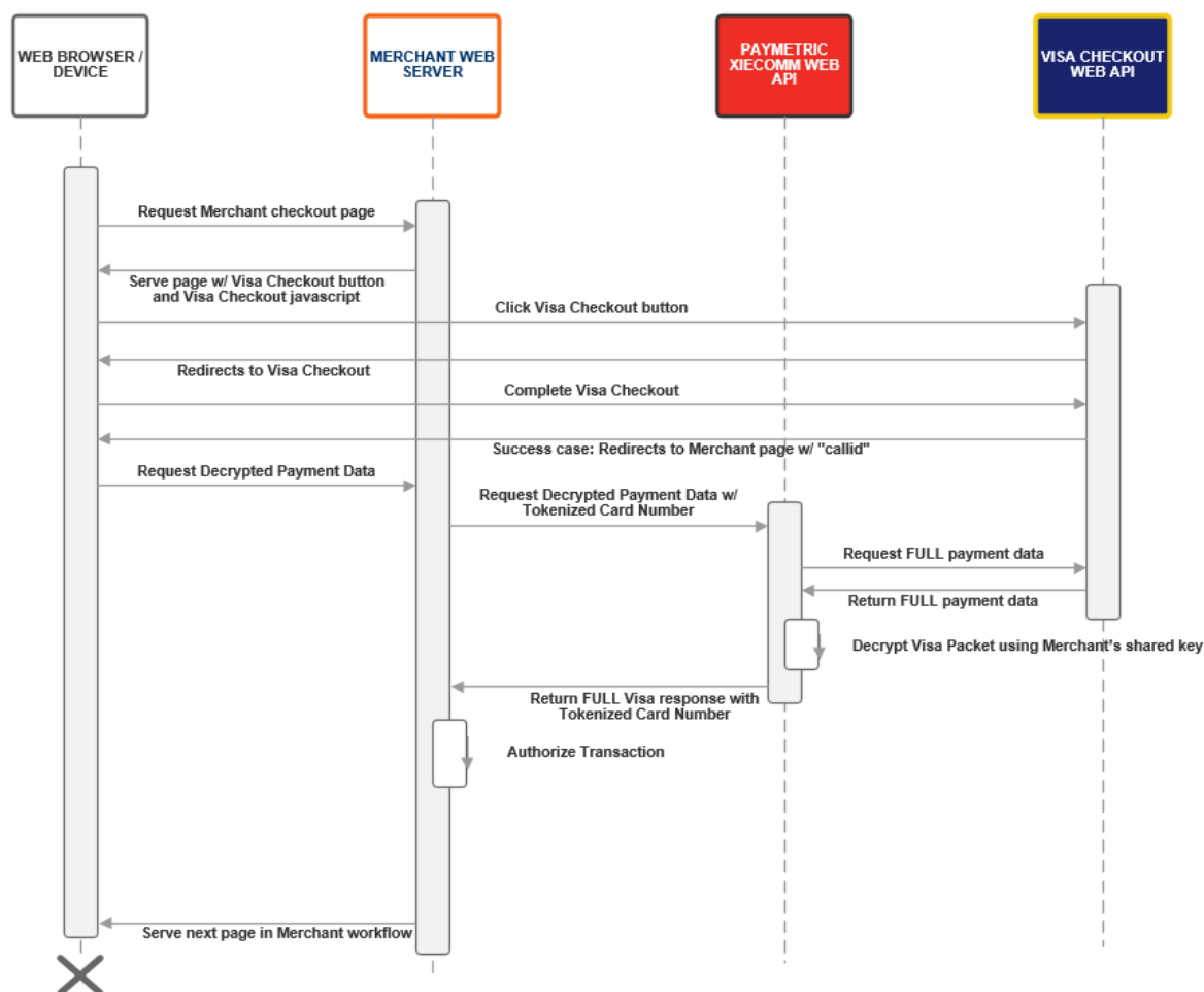
Figure 8: VisaCheckout Sequence Diagram
