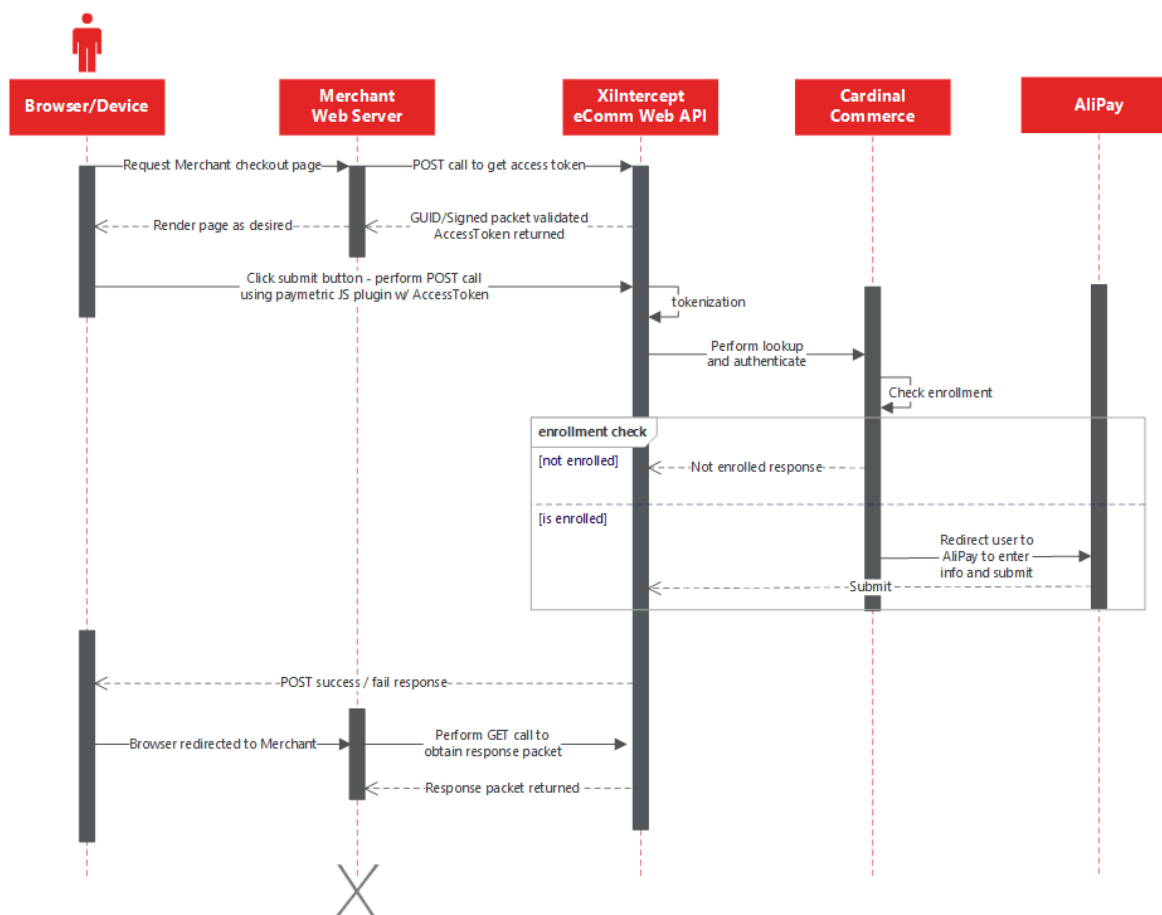
Figure 7: AliPay Integration Sequence Diagram
