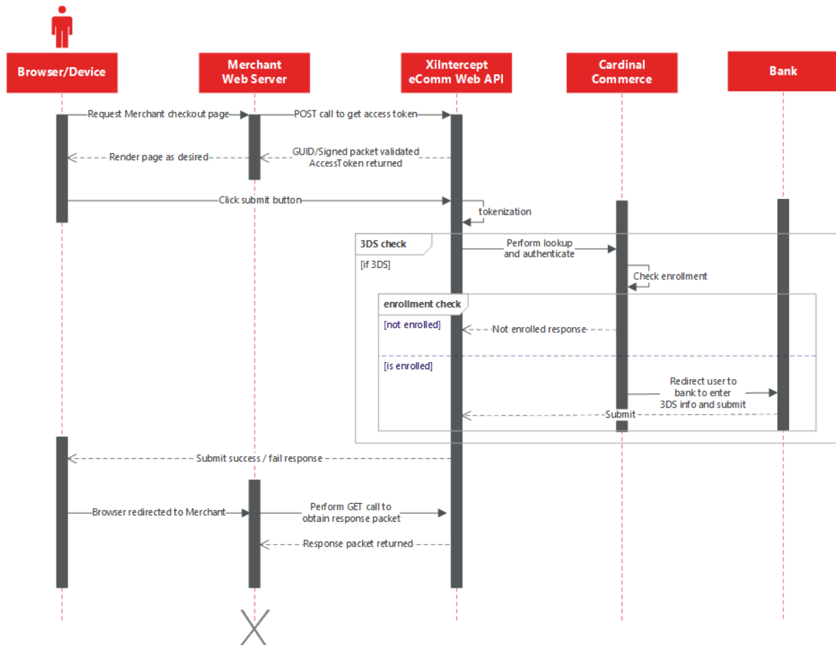
Figure 4: Hosted Integration Sequence Diagram
