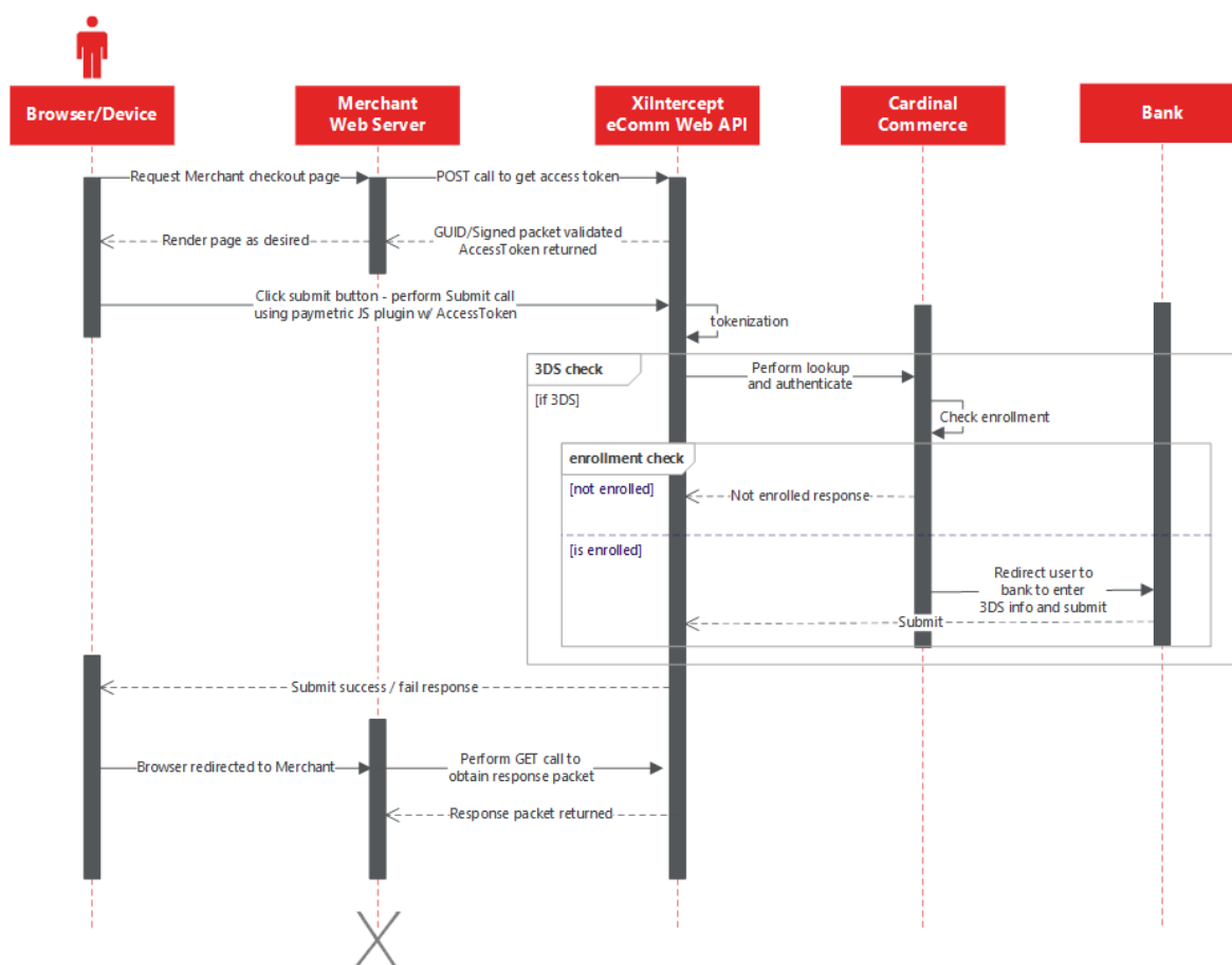
Figure 3: Iframe Integration Sequence Diagram
