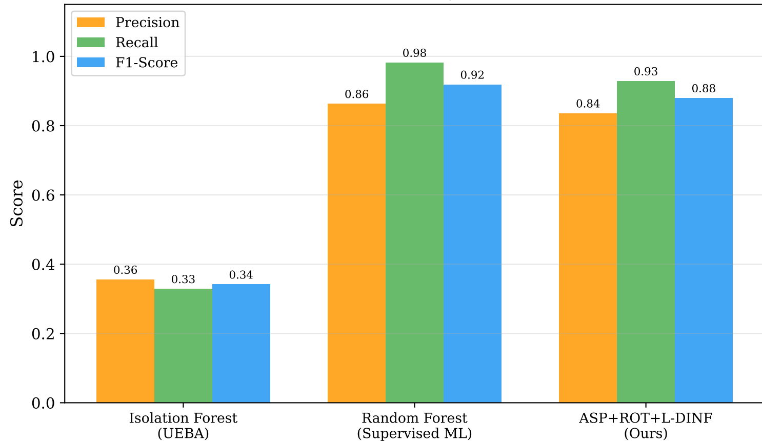
Detection Performance: Our System vs ML Baselines
