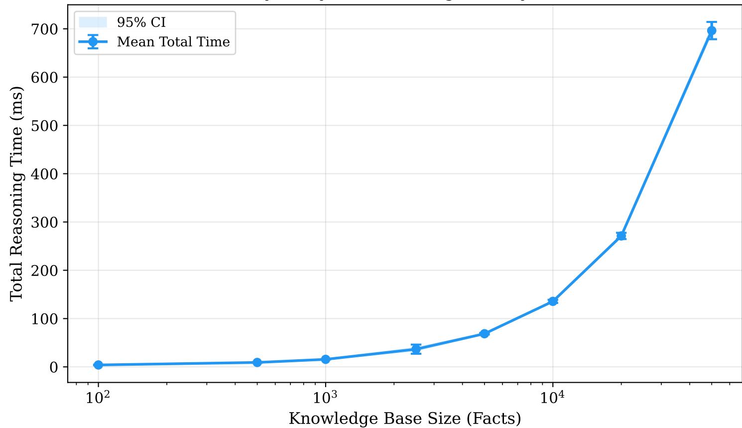
Scalability Analysis: Reasoning Latency vs KB Size
