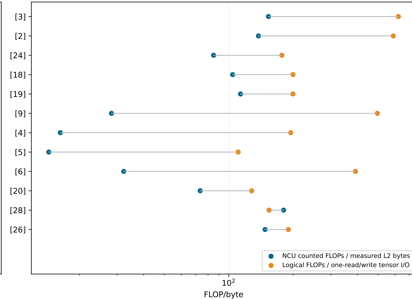
Memory-level choice changes arithmetic intensity
