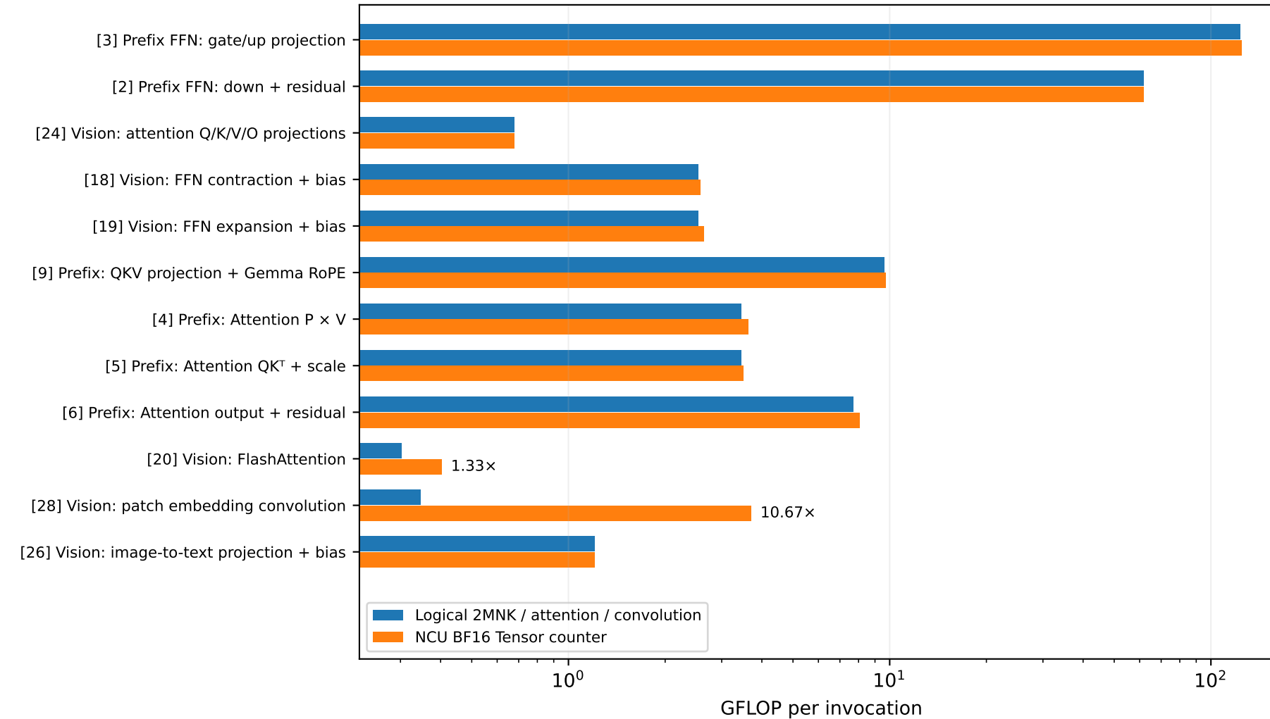
Useful Tensor work vs executed Tensor work
