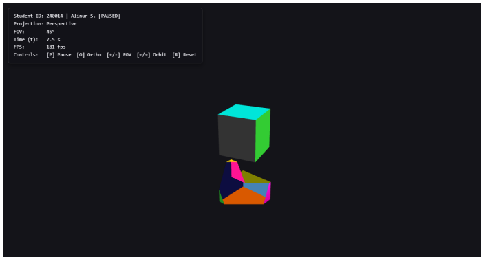
Fig. 3(a): Near Plane Clipping (near = 5.08 cuts staircase top)
