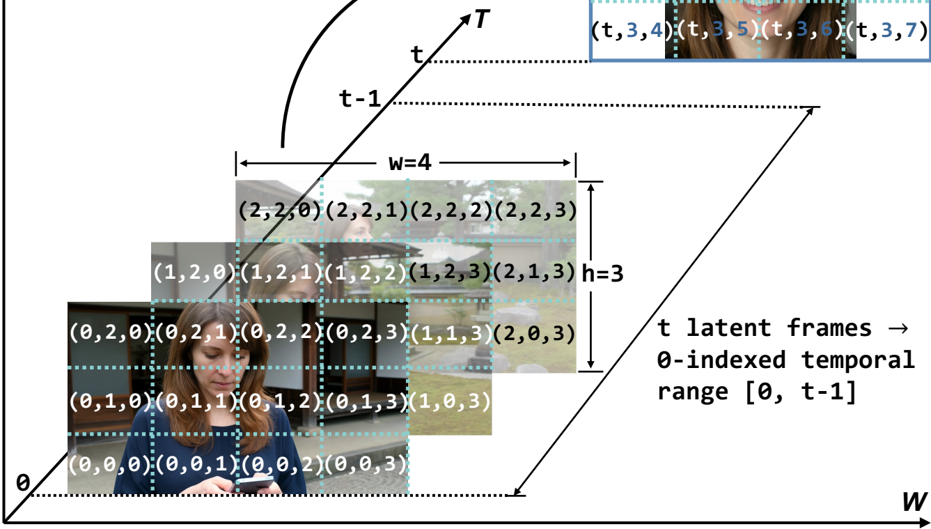
(b) TASS-RoPE Positioning
