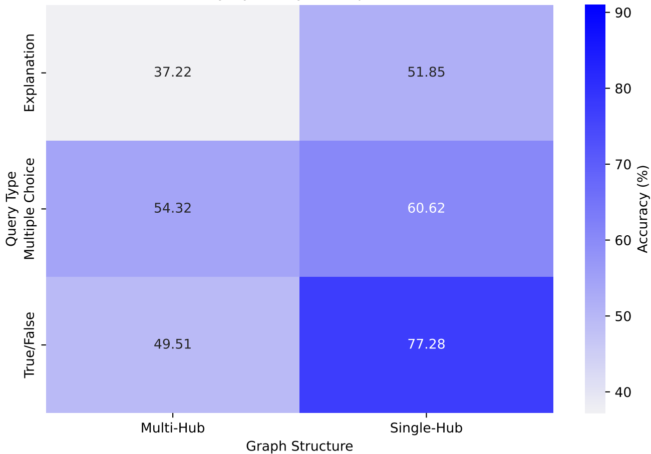
Accuracy by Query &amp; Graph (No KG)
