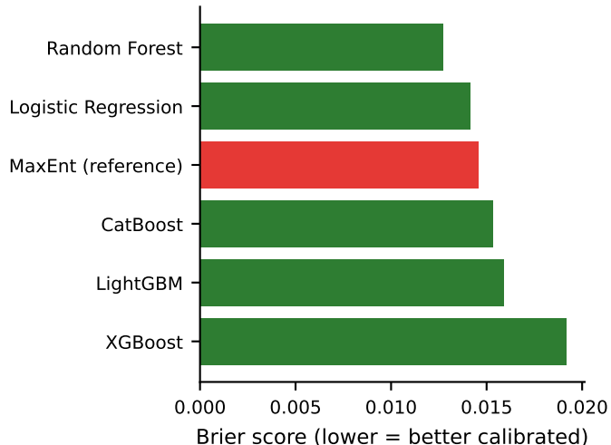
(b) Calibration (Brier score)
