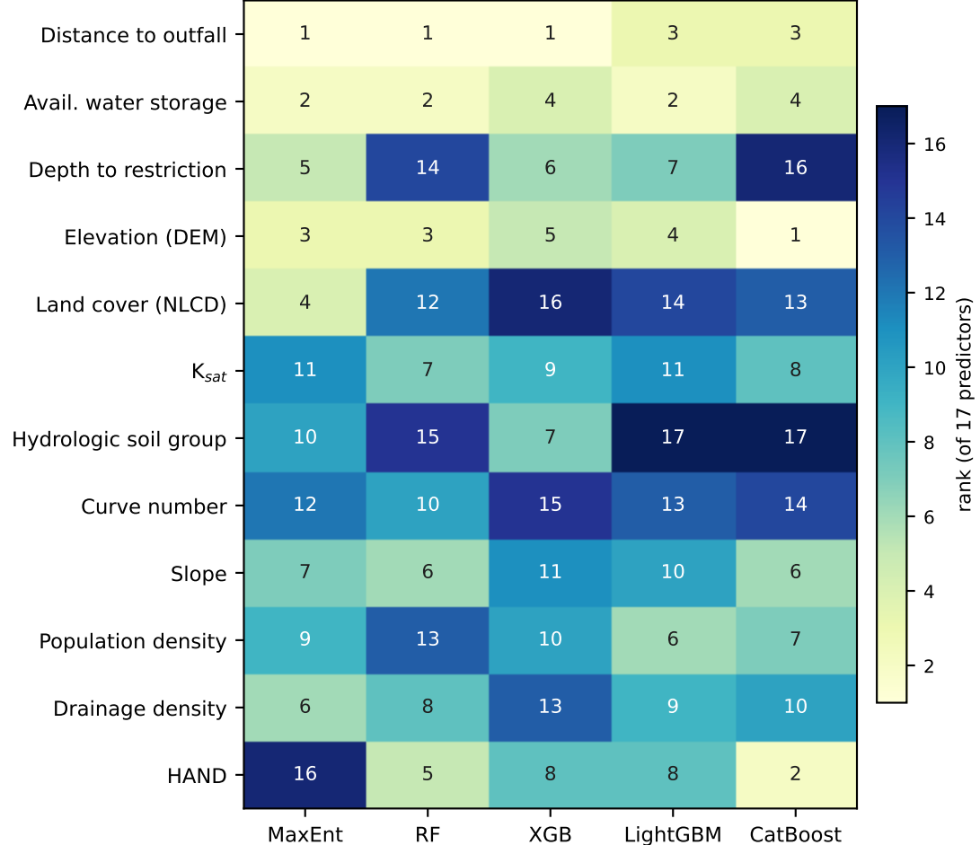
(b) Importance rank across models (1 = top)
