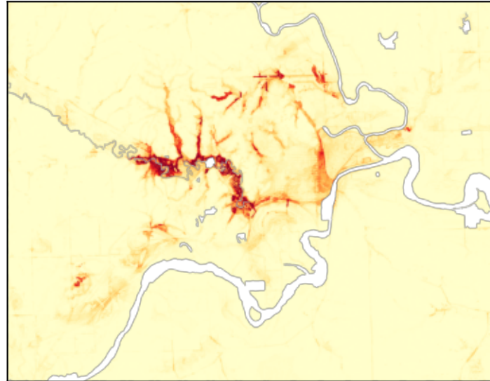
Random Forest (test AUC = 0.993)
