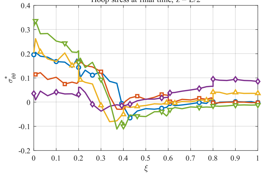
Hoop stress at final time, z = L/2
