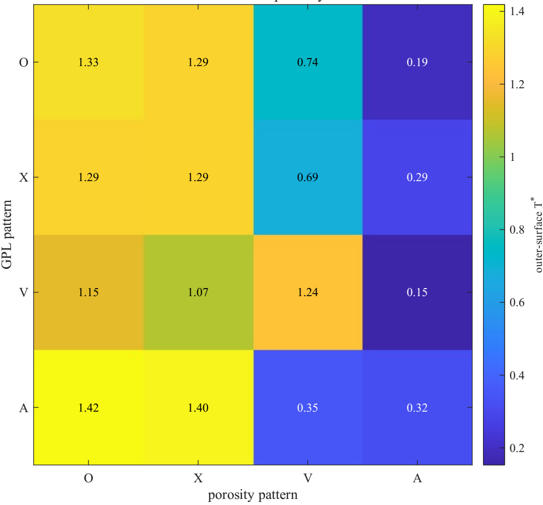
Outer-surface T^* : GPL \times porosity interaction
