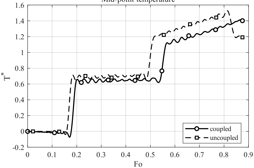
Mid-point temperature
