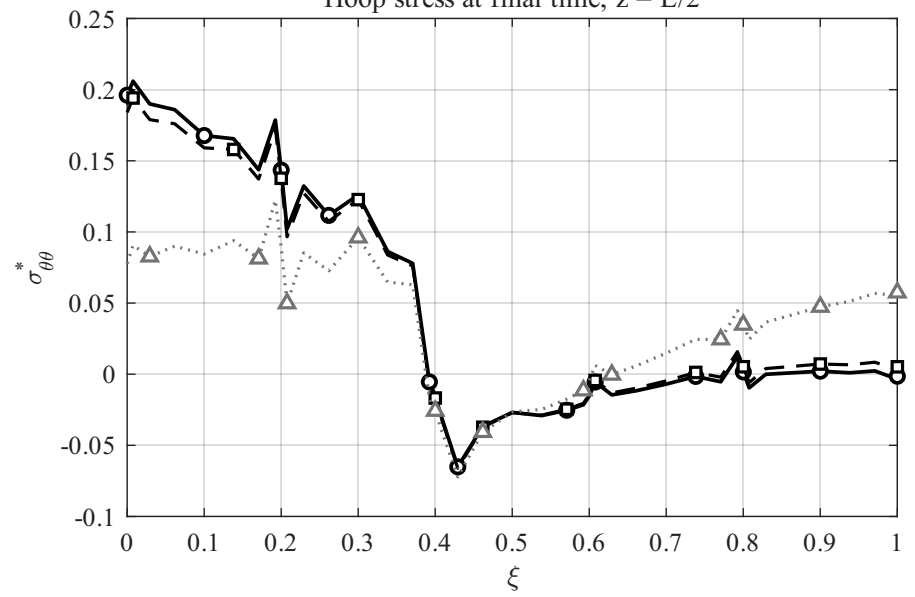
Hoop stress at final time, z = L/2
