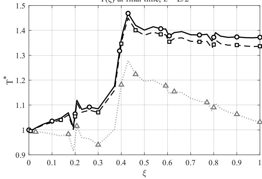
T(\xi) at final time, z = L/2
