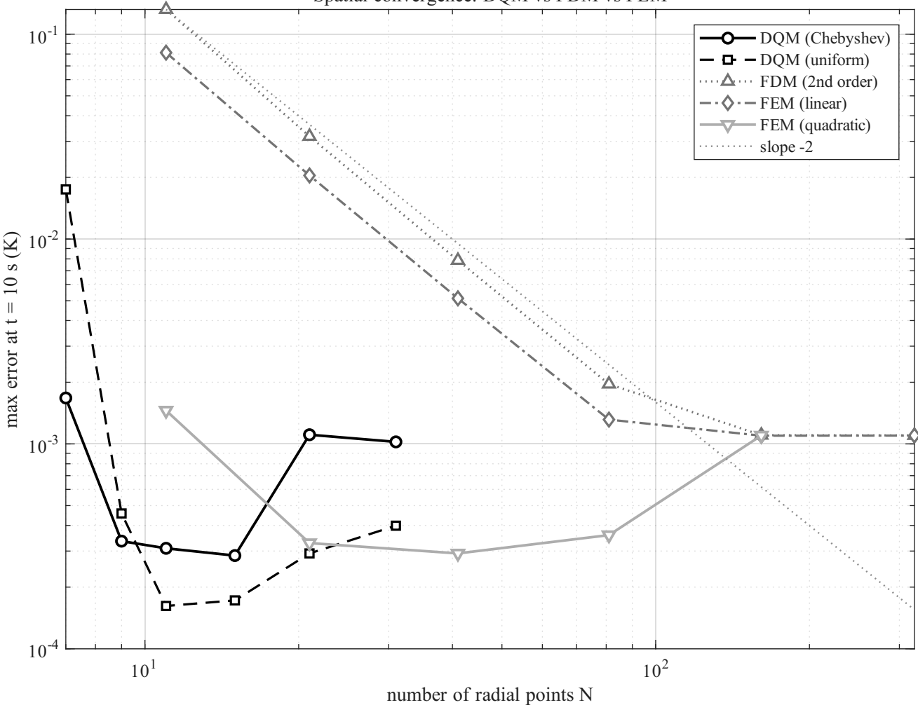
Spatial convergence: DQM vs FDM vs FEM
