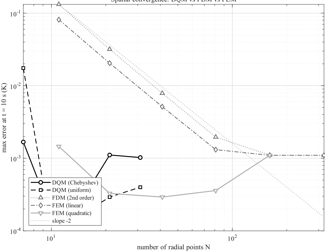
Spatial convergence: DQM vs FDM vs FEM
