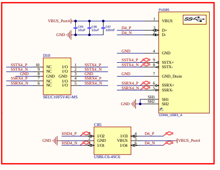
Port 4 Power Distribute
