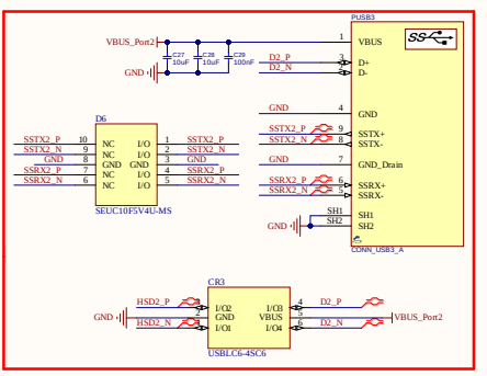
Port 2 Power Distribute
