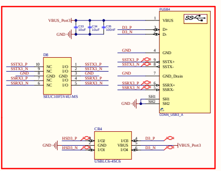
Port 3 Power Distribute
