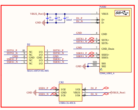
Port 1 Power Distribute
