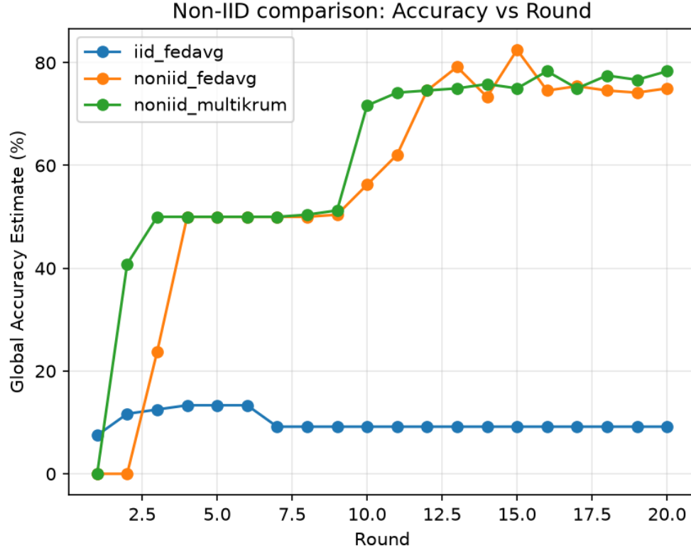
Figure 3: Non-IID comparison: federated-evaluation accuracy estimate vs. round (real data). The divergence between IID and Non-IID accuracy highlights the statistical challenge of highly skewed data distributions in federated settings.
