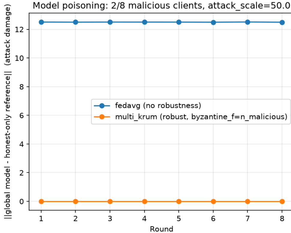
Figure 8: Poisoning attack damage per round: FedAvg vs. Multi-Krum (real data). The graph proves the effectiveness of Byzantine-robust strategies in fully neutralizing targeted adversarial poisoning.
