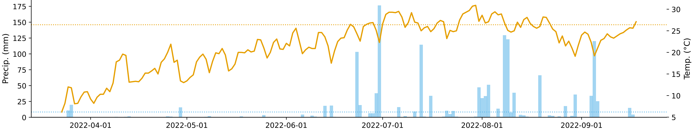
Panel C — Climate drivers
