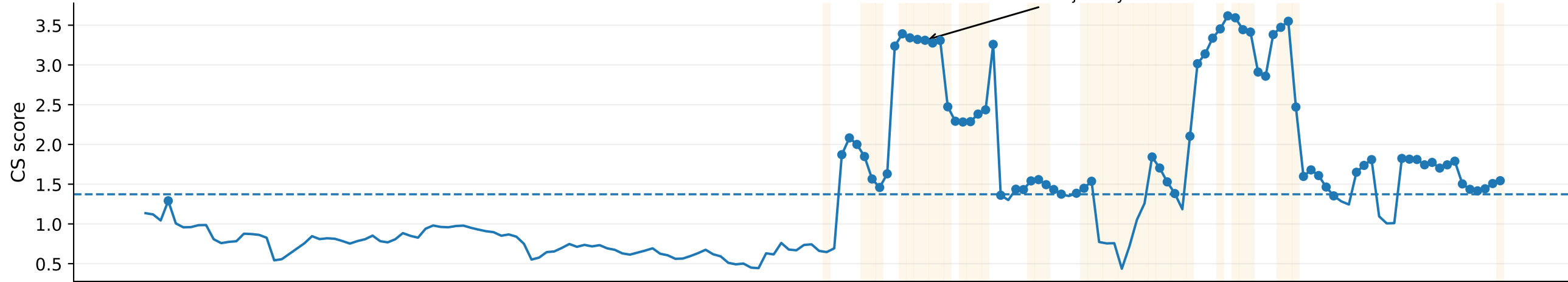
Panel B — Gaussian Copula
