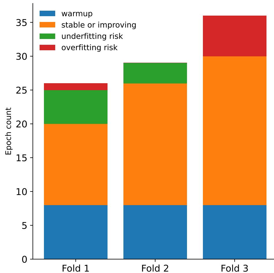
(B) Training-regime counts
