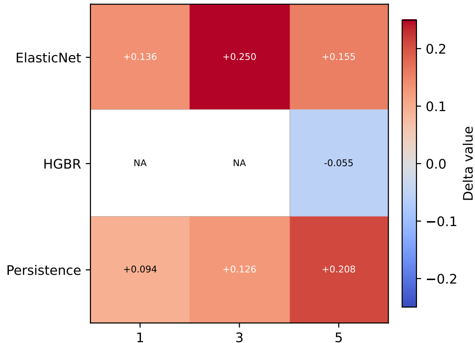
Alarm recall delta mean (Seoul - Ulsan)
