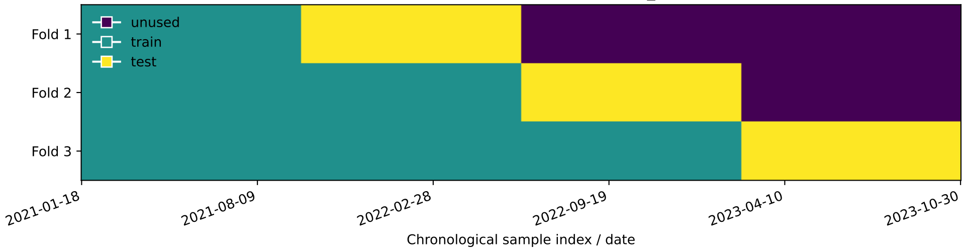
Blocked TimeSeriesSplit strategy (H=1, n_splits=3)
