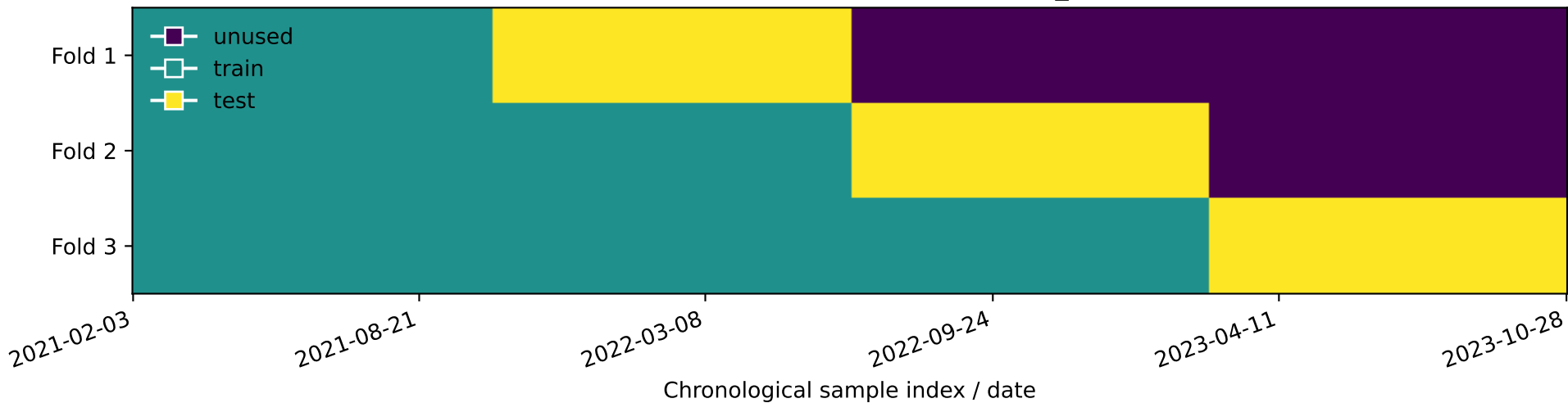
Blocked TimeSeriesSplit strategy (H=3, n_splits=3)
