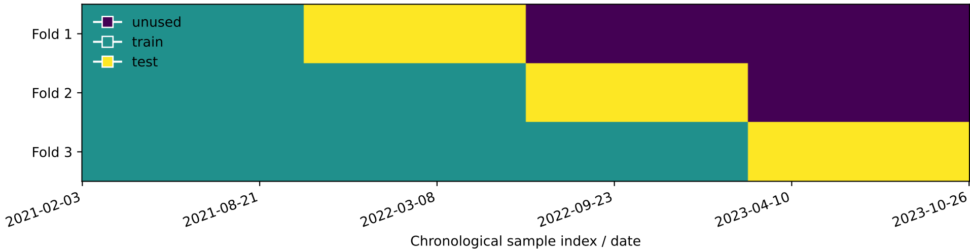
Blocked TimeSeriesSplit strategy (H=5, n_splits=3)
