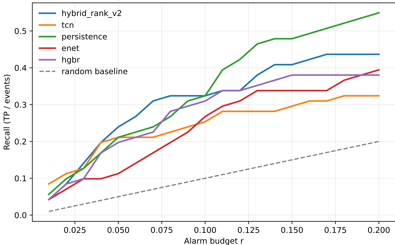
Budget-recall curve, TNout threshold \tau=16 , H=5
