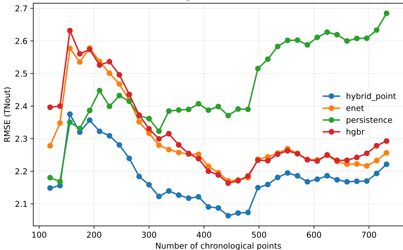
Learning curve (RMSE), H=5
