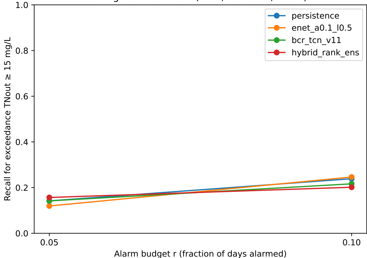
Budget-recall curve (H=5, Ulsan v2, \tau=15 )
