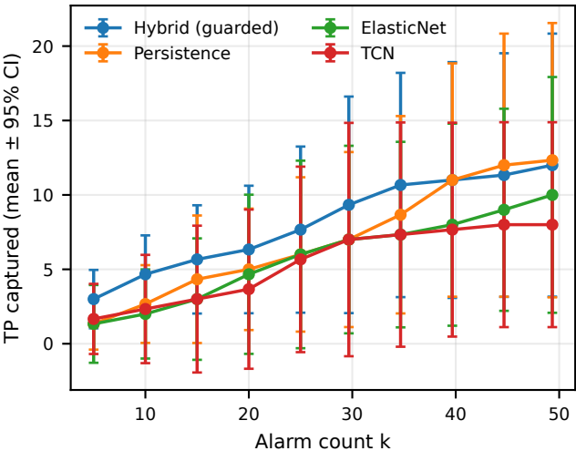
Decision curve at H=5 , \tau=16 mg/L
