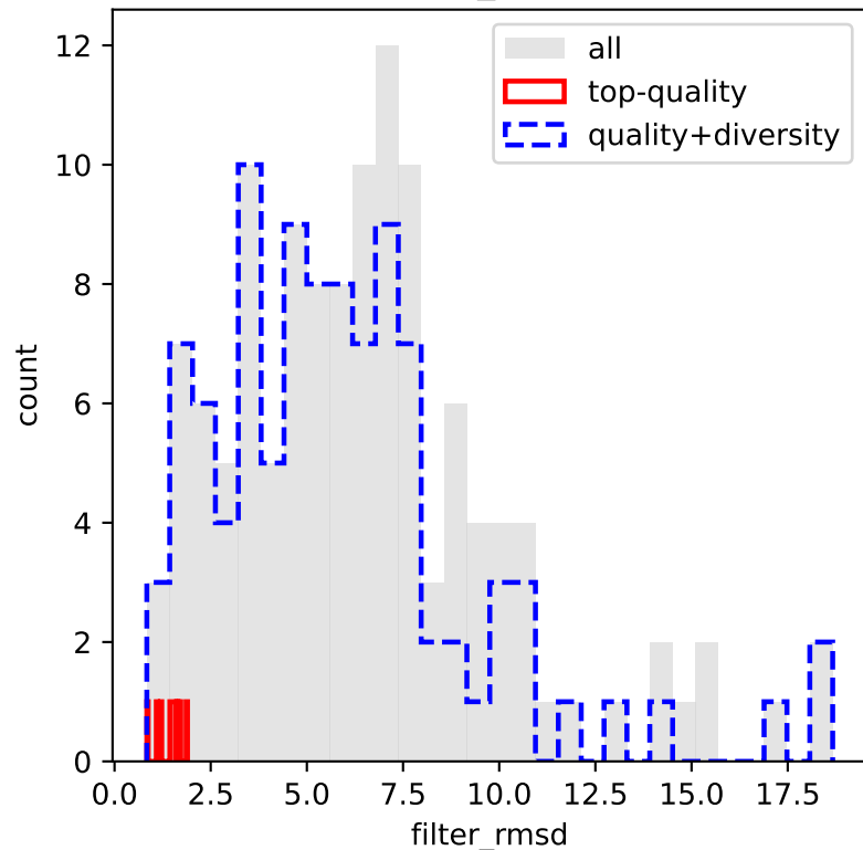
filter_rmsd
