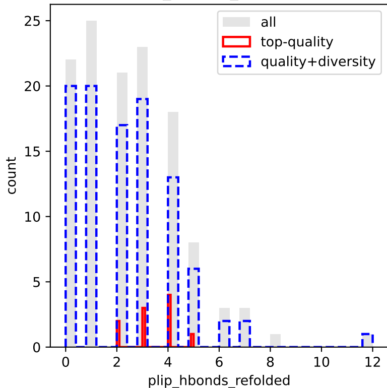
plip_hbonds_refolded
