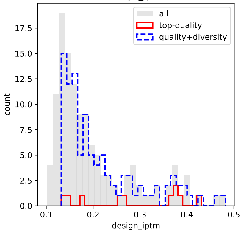
design_ipm
