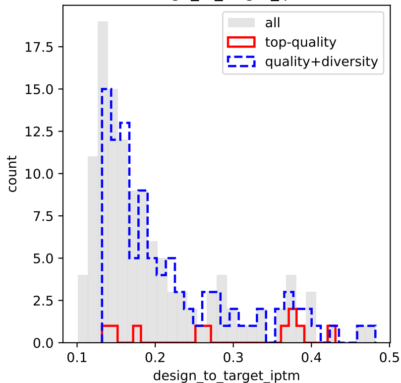
design_to_target_ip tm
